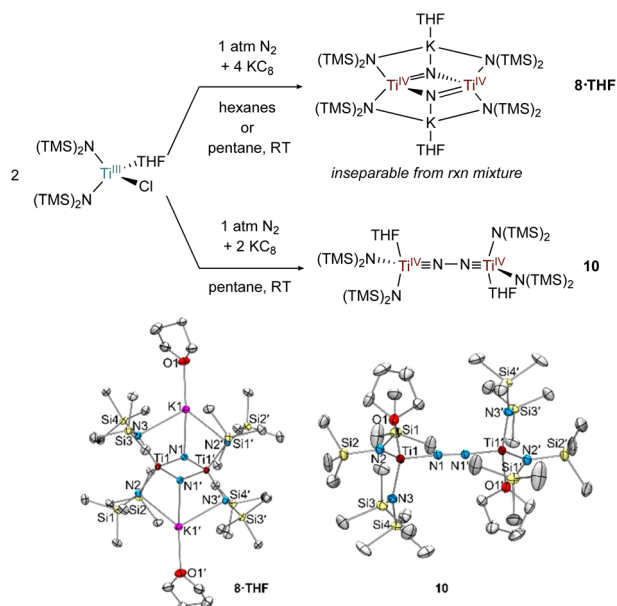
Fig. 10 1 : 2 reduction of [(\text{TMS})_2\text{N}]_2\text{TiCl}(\text{THF}) using \text{KC}_8 in the presence of \text{N}_2 generates 8 \cdot \text{THF} and a 1 : 1 reduction in pentane generates 10 (top). Crystal structures of 8 \cdot \text{THF} and 10 (bottom) with displacement ellipsoids at the 50% probability level. Hydrogen atoms and disorder were removed for clarity.
