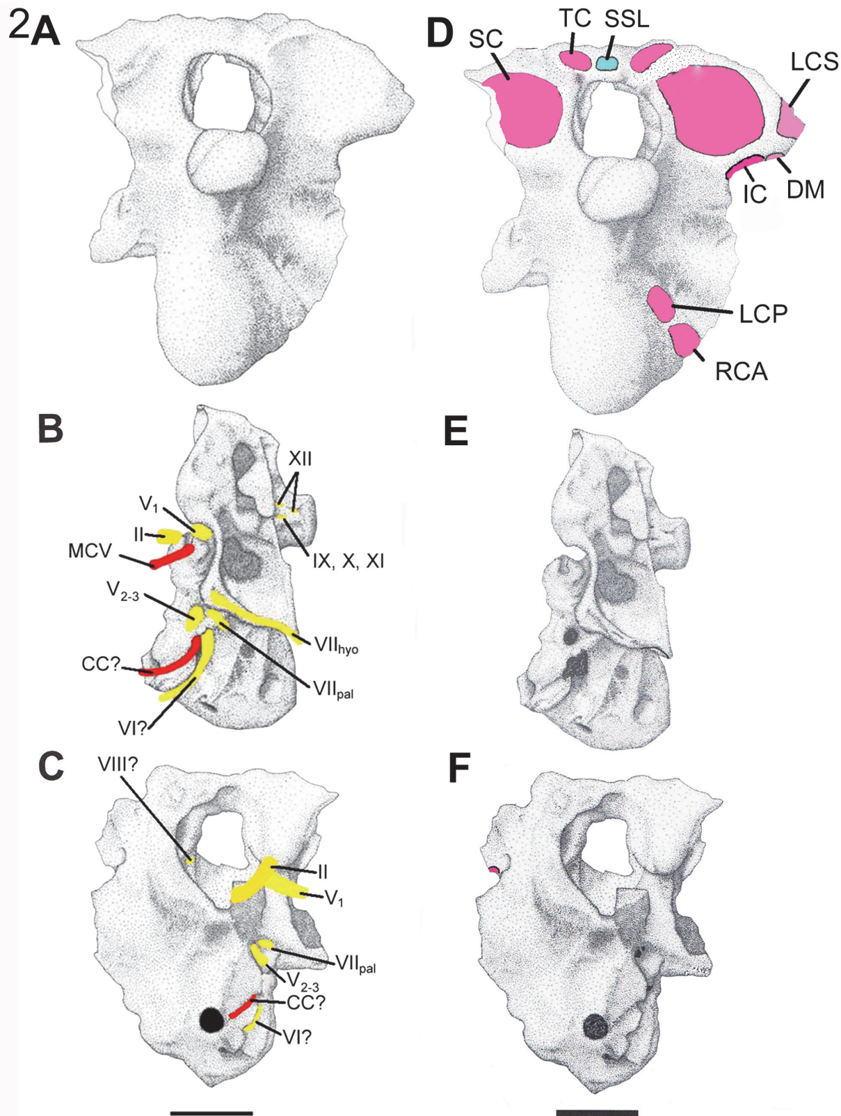
Fig 2. The braincase of Nothronychus mckinleyi (AzMNH P-2117), Turonian, Lower Cretaceous Moreno Hill Formation, west-central New Mexico in A, posterior; B, left lateral; and C, anterior views. Reconstructed nerves are indicated in yellow and blood vessels in red. The braincase of Nothronychus
