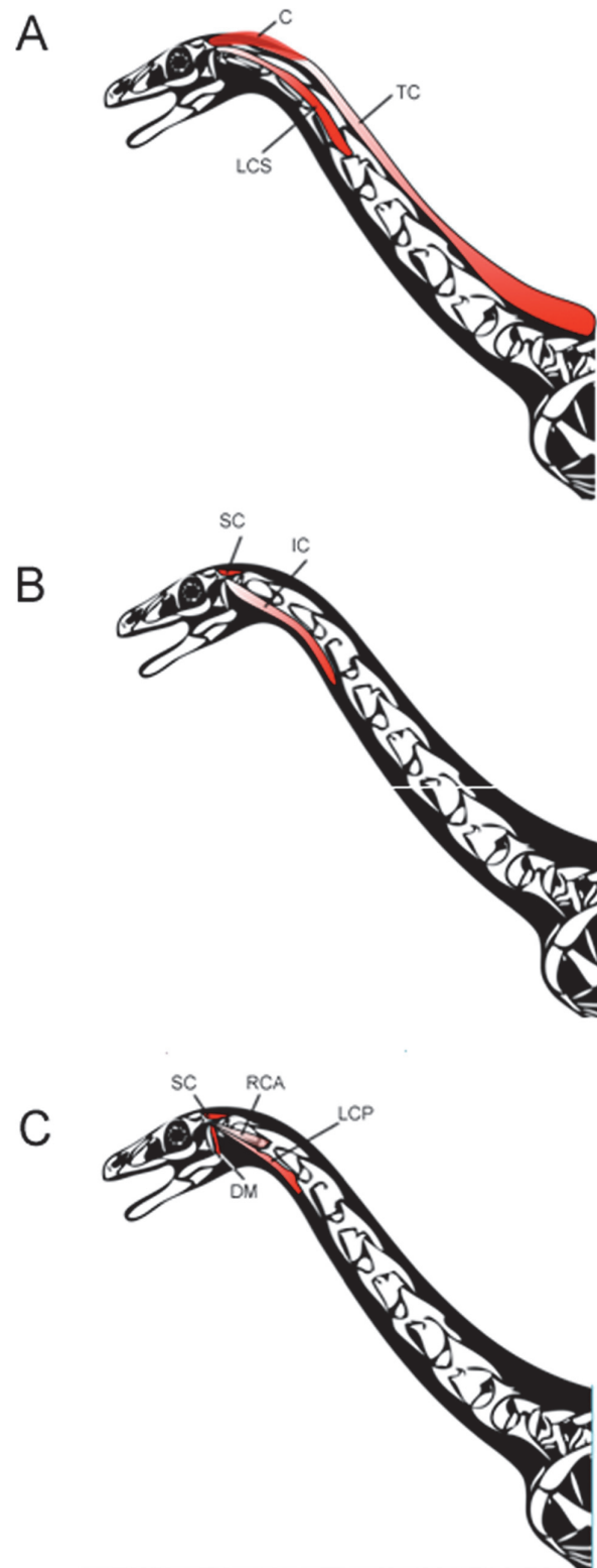
Fig 3. Reconstructed craniocervical musculature in the therizinosaur Falcarius utahensis and Nothronychus mckinleyi (after Scott Hartman, 2013). A, superficial; B, middle; and C, deep musculature. In the deep musculature, m. rectus capitis anterior would pass medial to the cervical ribs. Modifications by Eric Snively and David Smith.
