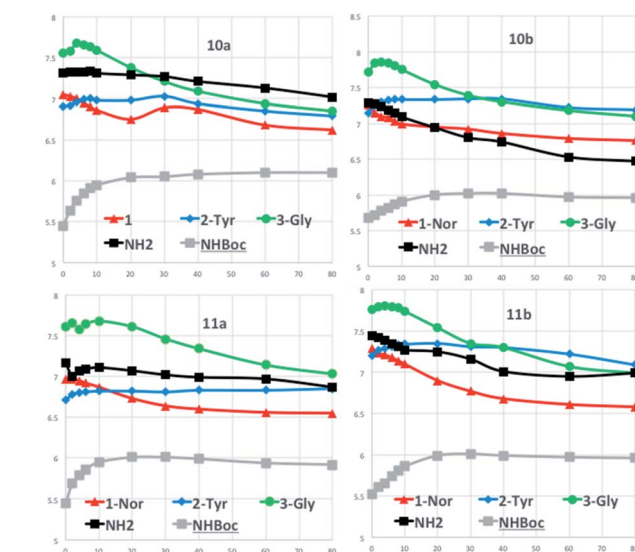
Fig. 4 DMSO-d 6 -titration of compounds 10a/11a and 10b/11b .
