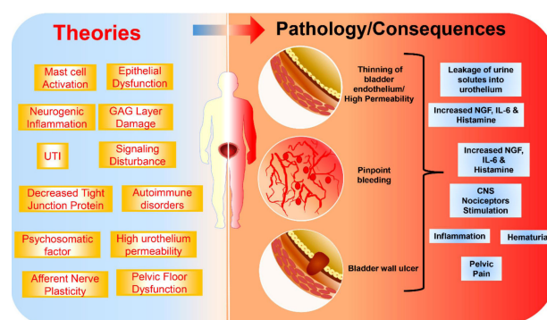
Fig. 1. IC/BPS Pathophysiology. GAG, glycosaminoglycan; UTI, urinary tract infections; NGF, nerve growth factor; IL-6, interleukin-6; CNS, Central nervous system. The figure is reproduced from the article by Dayem et al. 2020 (16). This article is an open access article distributed under the terms and conditions of the Creative Commons Attribution (CCBY) license ( http://creativecommons.org/licenses/by/4.0/ ).
