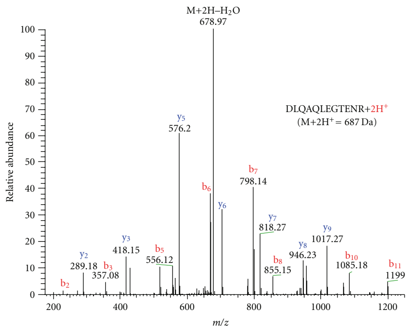
FIGURE 3: Fragmentation pattern of the doubly charged peptide DLQAQLEGTENR (residues 135 to146) from the protein LemA. This peptide covers 5.6% of the protein sequence and 5 additional unique peptides of this protein were found in the extra cellular fraction of B. vietnamiensis G4.
