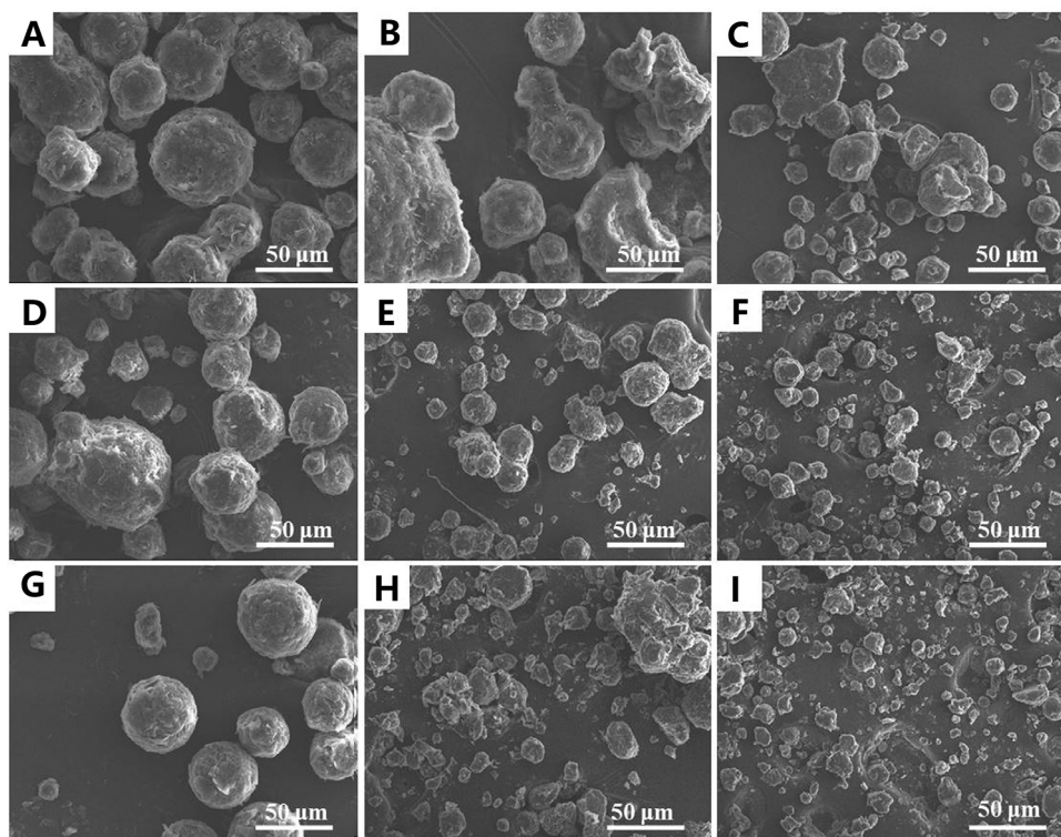
Fig. 4 - SEM characteristics demonstrated the morphology of ibuprofen microspheres at different sampling times. (A, B, and C) are images of air-cooling microspheres (ACM) at 0, 5, 10 min; (D, E, and F) are images of water-cooling microspheres (WCM) at 0, 5, 10 min; (G, H, and I) are images of citric acid solution-cooling microspheres (CCM) at 0, 5, 10 min.
