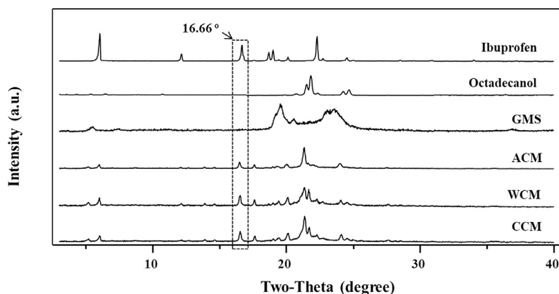
Fig. 2 – XRD characteristics illustrated the components in microspheres. GMS: glycerin monostearate; ACM: air-cooling microspheres; WCM: water-cooling microspheres; CCM: citric acid solution-cooling microspheres.
