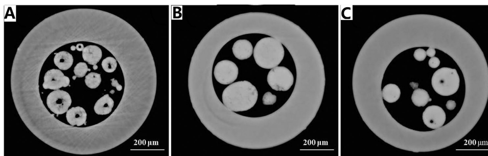
Fig. 5 – 2D slice pictures of three kinds of ibuprofen microspheres. (A) air-cooling microspheres (ACM); (B) water-cooling microspheres (WCM); (C) citric acid solution-cooling microspheres (CCM).
