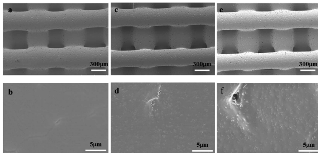
Fig. 1 SEM images: PCL scaffold at 300 \mu\text{m} (a), PCL scaffold at 5 \mu\text{m} (b), PCL/HA scaffold at 300 \mu\text{m} (c), PCL/HA scaffold at 5 \mu\text{m} (d), EPL/PCL/HA scaffold at 300 \mu\text{m} (e), EPL/PCL/HA scaffold at 5 \mu\text{m} (f).
