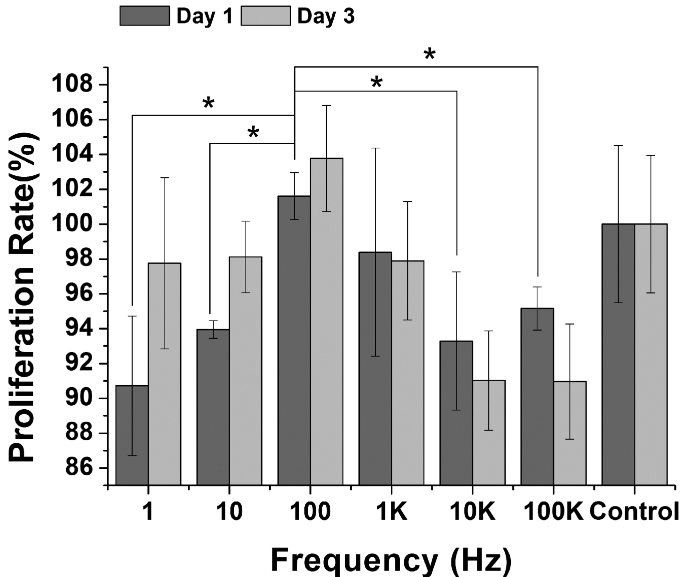
Fig 2. Assessment of Proliferation in MC-3T3-E1 cells after ES. MTT assay to assess proliferation of the MC-3T3-E1 cells after ES. 100 Hz group has the highest proliferation rate at days 1, 3 compared to the other frequency and control group. 1K Hz group showed similar proliferation compared to control group at days 1, 3. 1 Hz, 10 Hz, 10 KHz, and 100 KHz showed lower proliferation than control group at day 1. ( P < 0.05 , indicated statistically significant difference)
