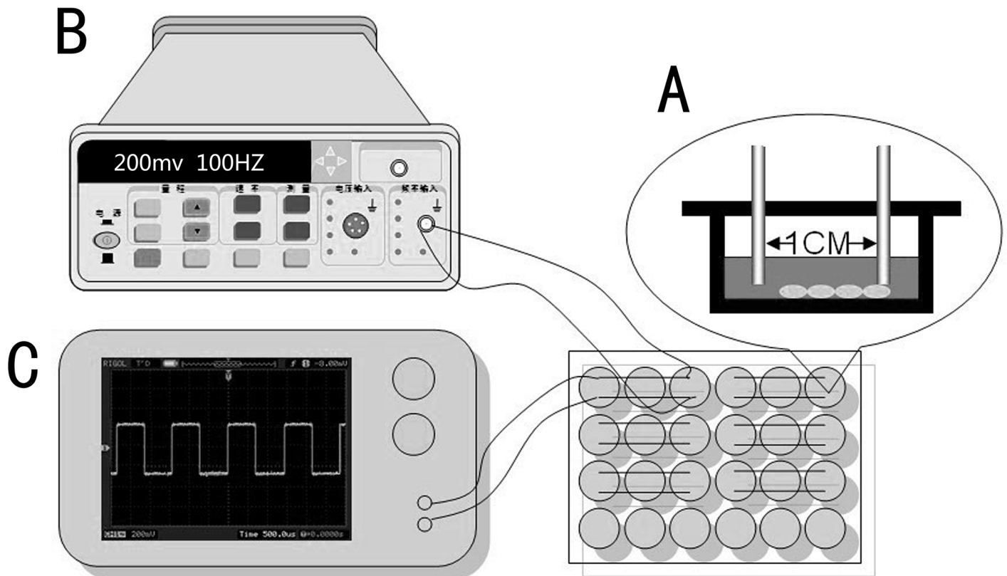
Fig 1. Chamber design and ES setup. (A) Platinum electrode chamber design for direct coupling; (B) ES setup including signal function generator for power supply; (C) Oscilloscope for ES verification.
