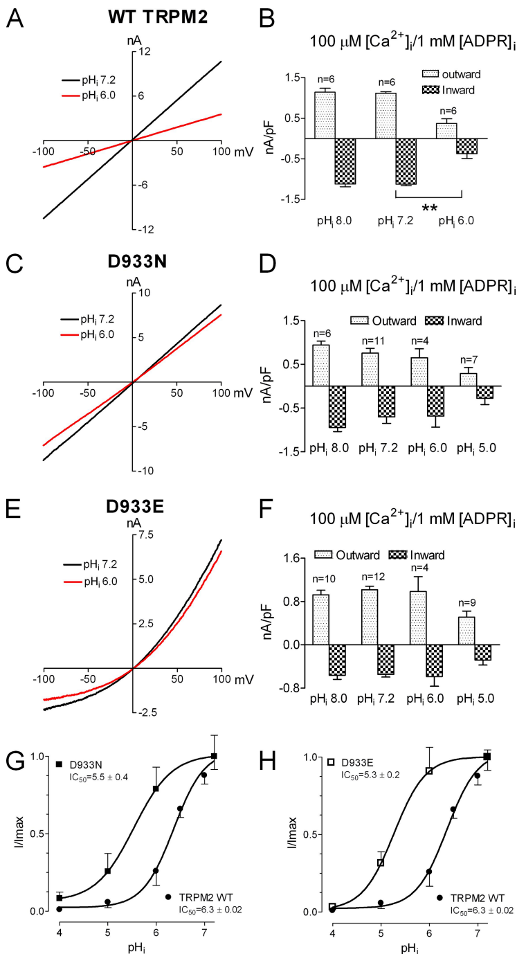
Figure 13. D933 is an intracellular pH sensor. (A and B) WT TRPM2 activated by 100 μM [Ca 2+ ] i /1 mM [ADPR] i was largely blocked at pH i 6.0. (C and D) Effects of acidic pH i on D933N activated by 100 μM [Ca 2+ ] i /1 mM [ADPR] i . Acidic pH i 6.0 did not change current amplitude, whereas pH i 5.0 significantly inhibited D933N currents. (E and F) Effects of pH i on D933E. A significant decrease in current amplitude was observed at pH 5.0, but not pH 6.0. (G and H) Concentration-dependent effects of acidic pH i on D933N and D933E. IC 50 s obtained by best fit of the dose-response curves were 5.5 ± 0.4 pH units for D933N and 5.3 ± 0.2 pH units for D933E. **, P < 0.01.
