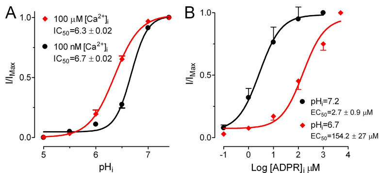
Figure 11. Effects of internal protons on [Ca^{2+}]_i - and [ADPR]_i -induced TRPM2 gating. (A) Concentration-dependent effects of internal protons on TRPM2 at various concentrations of internal [Ca^{2+}]_i . TRPM2 currents were elicited by voltage ramps ( -100 to +100 mV; HP = 0 mV) under inside-out configuration, and the macroscopic current amplitude was measured at +100 mV. The intracellular solution (bath solution) contained 200 \mu M ADPR with 100 \mu M or 100 nM Ca^{2+} ; the external solution (pipette solution) was normal Tyrode's solution containing 2 mM Ca^{2+} . Best fit of normalized current yielded an IC_{50} of 6.7 \pm 0.02 ( n = 10 ) at 100 nM [Ca^{2+}]_i and 6.3 \pm 0.02 ( n = 11 ; P < 0.01 ) at 100 \mu M [Ca^{2+}]_i . (B) Effects
