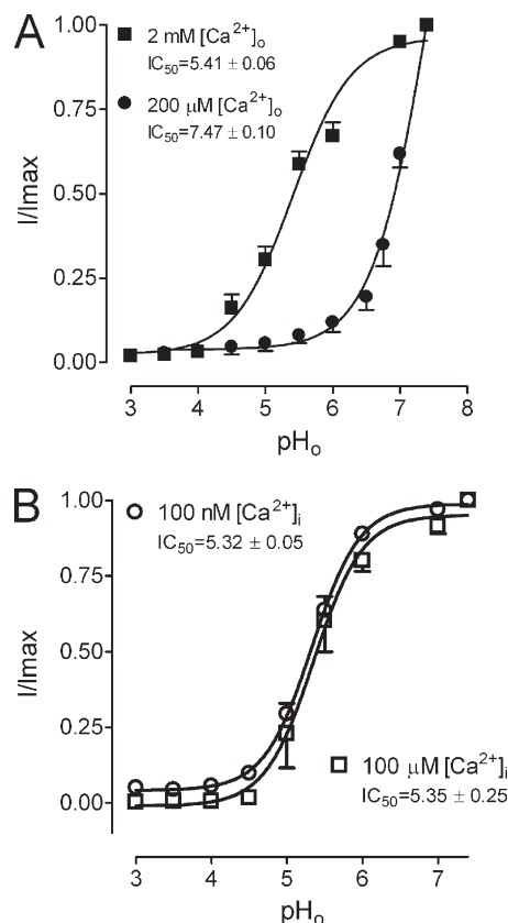
Figure 3. Effects of external and internal Ca^{2+} on protons' inhibition of TRPM2. (A) Concentration-dependent effects of external acidic pH on TRPM2 in the solutions containing 200 \mu M and 2 mM [Ca^{2+}]_o , respectively. Whole cell currents were recorded with pipette solutions containing minimal [Ca^{2+}]_i buffered by 10 mM EGTA and 500 \mu M ADPR. Ramp protocol ( -100 to +100 mV) was used to elicit TRPM2 currents. Current amplitude at +100 mV was measured and normalized to the maximal current amplitude at pH 7.4. The proton dose–response curve was rightward shifted at 200 \mu M of external [Ca^{2+}]_o , and the IC_{50} was changed from 5.4 \pm 0.05 pH units (2 mM [Ca^{2+}]_o ; n = 8 ) to 7.5 \pm 0.1 pH units (200 \mu M [Ca^{2+}]_o ; n = 8 ). (B) Effects of internal [Ca^{2+}]_i on concentration-dependent inhibition of TRPM2 by external protons. Whole cell currents of TRPM2 were recorded in the 2 mM of external Ca^{2+} with pipette solutions containing 100 nM or 100 \mu M [Ca^{2+}]_i in the presence of 200 \mu M [ADPR]_i . Protons produced similar inhibitory effects on TRPM2 at 100 nM ( n = 9 ) and 100 \mu M ( n = 6 ) of internal [Ca^{2+}]_i (with 200 \mu M ADPR), respectively.
