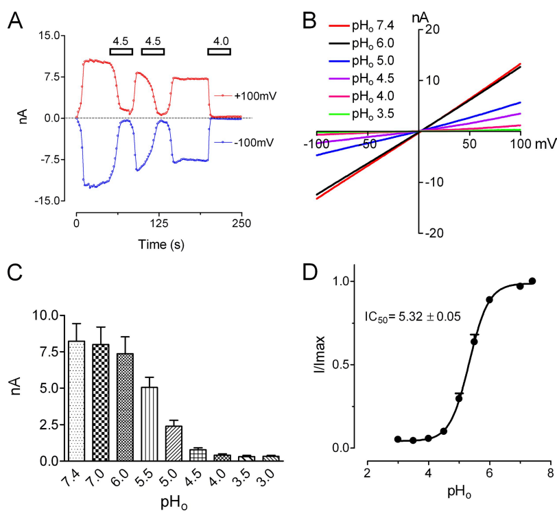
Figure 1. Inhibitory effects of acidic pH o on TRPM2. (A) Both inward and outward currents of TRPM2 elicited by voltage ramps ranging from –100 to +100 mV were completely and reversibly inhibited by pH o 4.5. Note that pH o 4.0 irreversibly blocked TRPM2. Internal pipette solutions contained 100 nM [Ca 2+ ] i buffered by 1 mM EGTA and 200 μM ADPR. Inward and outward currents were measured at –100 and +100 mV, respectively. (B) Representative recordings of TRPM2 by ramp protocols ranging from –100 to +100 mV at the indicated pH o . (C) Mean current amplitude of TRPM2 at the indicated pH o (mean ± SEM; n = 9 ). (D) Dose–response curve of pH o constructed by normalizing current amplitude at the indicated pH o to the maximal current amplitude at pH o 7.4. Best fit of the normalized data yielded an IC 50 of 5.3 \pm 0.05 pH units (mean ± SEM; n = 9 ; Hill coefficient, n_H = 1.3 ).
