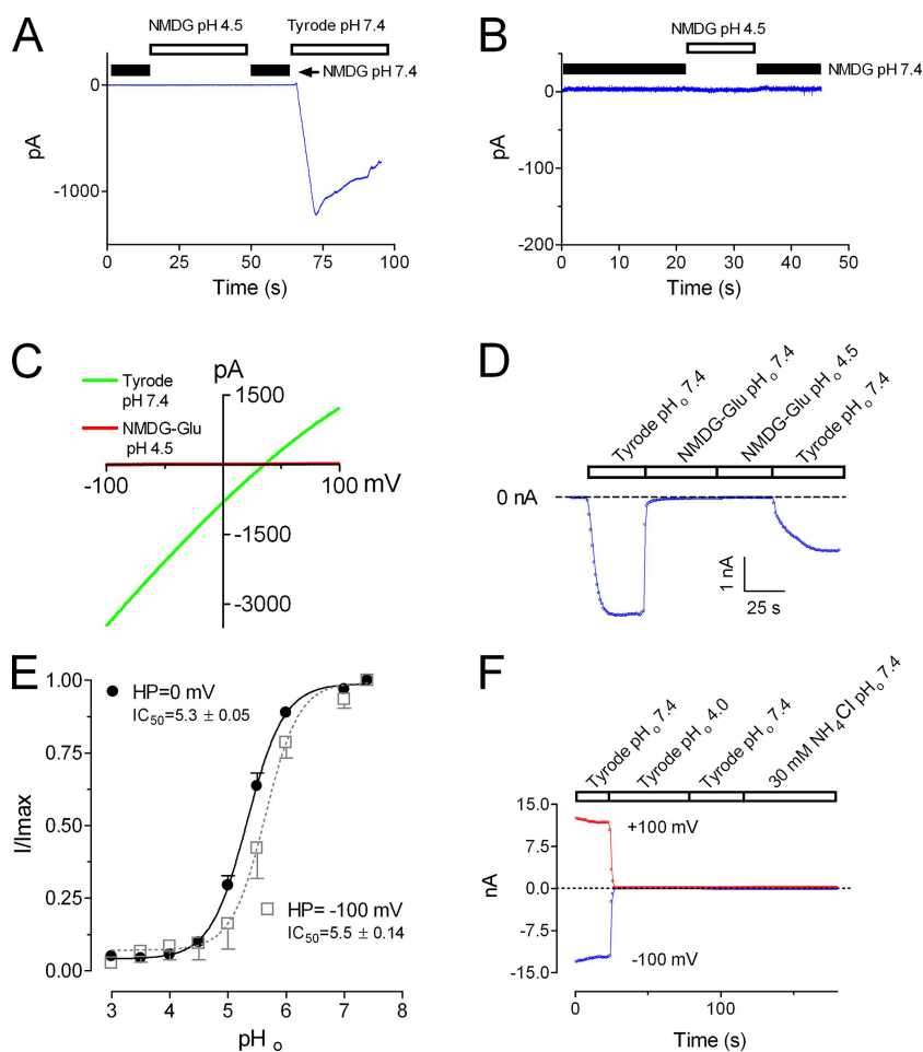
Figure 4. TRPM2 is not permeable to protons. (A) Inward currents of TRPM2 recorded by holding the TRPM2-transfected cell at -100 mV. No current was activated in NMDG-Glu solutions at pH o 4.5 or 7.4, where Tyrode's solution generated large inward current. (B) In mock-transfected cells, NMDG-Glu solutions at pH o 4.5 or 7.4 could not induce any current. (C) TRPM2 current elicited by the ramp protocol (-100 to +100 mV) in Tyrode's solution (red). NMDG-Glu at pH o 4.5 did not induce any inward proton current (green). The pipette solution for this experiment contained NMDG-Glu to favor proton permeation. (D) Inward current of TRPM2 recorded at various external solutions obtained in C. Currents were measured at -100 mV and plotted as a function of time. (E) Effects of holding potentials on the inhibition of TRPM2 by external protons. Dose-response curves were constructed by normalizing the inward currents (-100 mV) at each pH o to the maximal current amplitude (-100 mV) obtained at pH o 7.4. The IC 50 s were 5.3 ± 0.05 ( n = 9) at HP = 0 mV and 5.5 ± 0.14 ( n = 9; P > 0.05) at HP = -100 mV. (F) Inhibition of TRPM2 by acidic pH o (pH o = 4.0) could not be reversed by high pH i . Inward currents (-100 mV) and outward currents (+100 mV) plotted against time under the indicated conditions. TRPM2 currents were elicited by voltage ramps with the CsSO 3 CH 3 pipette solution containing 100 nM Ca 2+ and 200 μM ADPR. Note that TRPM2 was completely and irreversibly blocked by external solutions at pH o 4.0. 30 mM NH 4 Cl, used to increase intracellular pH, could not reverse the effects of pH o 4. Similar results were obtained in five separate experiments.
