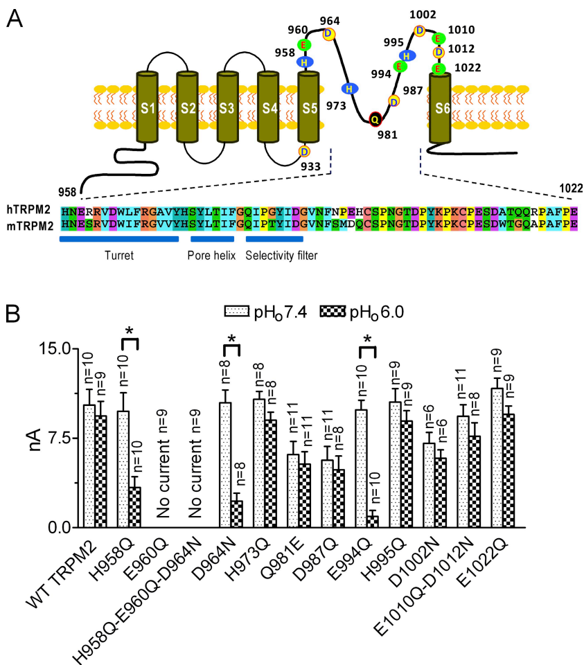
Figure 5. Molecular basis for TRPM2 sensitivity to acidic pH o . (A) Schematic structure of TRPM2 and positions of substituted amino acid residues in the putative pore region of hTRPM2 (top). Alignment of the residues in the putative pore region of mTRPM2 and hTRPM2 (bottom). (B) Average current amplitude of WT TRPM2 and the mutants at pH o 7.4 and 6.0. TRPM2 currents were elicited by voltage ramps, and the outward currents at +100 mV were measured. E960Q and the triple mutant H958Q-E960Q-D964N were nonfunctional channels. *, P < 0.05.
