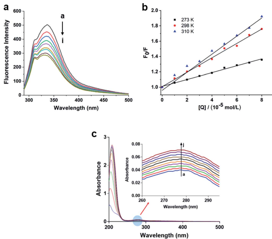
Fig. 5 (a) Fluorescence emission spectra of \alpha -glucosidase in the presence of various concentrations of compound 6 . The concentration of compound 6 increases from (a) to (i) ( 0, 1, 2, 3, 4, 5, 6, 7, 8 \times 10^{-5} \text{ mol L}^{-1} ). (b) Simple Stern–Volmer plot of the quenching of \alpha -glucosidase fluorescence by compound 6 at different temperatures (273 K, 298 K, and 310 K). (c) UV-Vis absorption spectra of \alpha -glucosidase in the presence of various concentrations of compound 6 . The concentration of compound 6 increases from (a) to (j) ( 0, 1, 2, 3, 4, 5, 6, 7, 8, 9 \times 10^{-5} \text{ mol L}^{-1} ).
