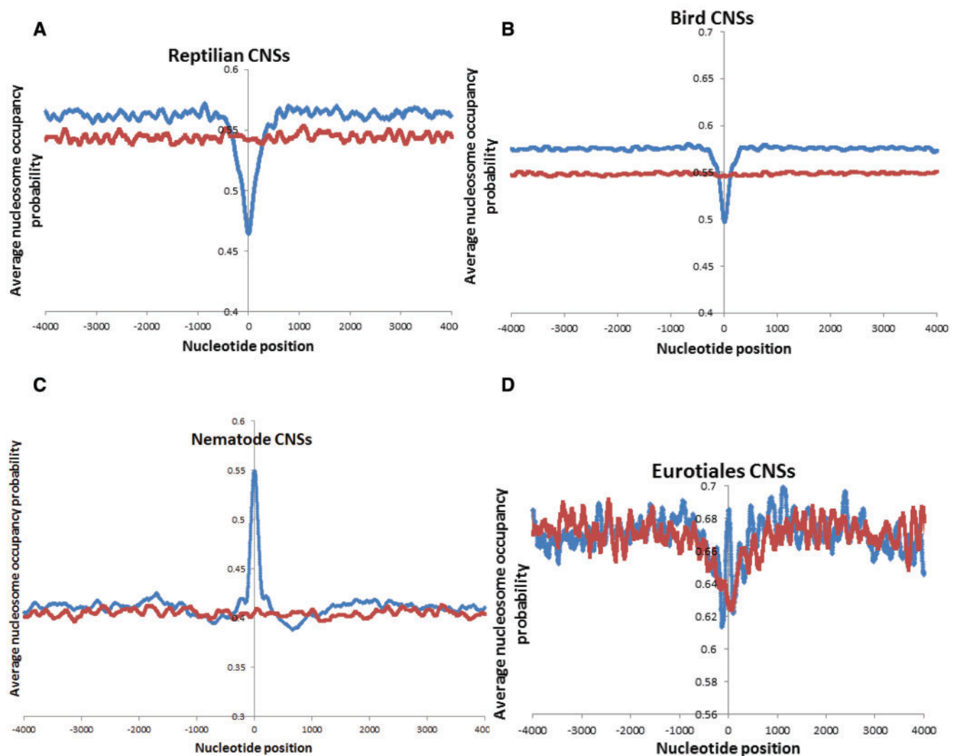
Fig. 4. —Nucleosome occupancy probability for the CNSs of different lineages. The 0th position represents the center of the CNSs. 8000bp flanks were considered for this analysis. The blue and red colors represent the nucleosome occupancy for CNSs and random samples, respectively. (A) Reptilian CNSs average nucleosome occupancy probability, (B) bird CNSs average nucleosome occupancy probability, (C) Nematode CNSs average nucleosome occupancy probability, and (D) Eurotiales CNSs average nucleosome occupancy probability. (The statistical significance between the center 1000 bases of CNSs and center 1000 bases of random sequences for Reptilian, bird, Nematode, and Eurotiales are 2.37\text{E-}81 , 0.00 , 9.78\text{E-}73 , and 3.87\text{E-}22 , respectively.).
