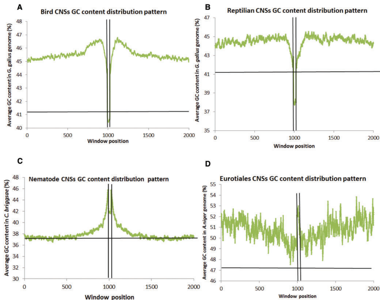
FIG. 3. —GC content distribution of the CNSs across the center of CNSs and the flanking regions. The 1000th nucleotide position corresponds to the center of the CNSs. The horizontal back line represents the level of non-coding GC content of the reference genome. The vertical lines represent the margins of the flanking regions. (A) bird CNSs GC distribution. (B) Reptilian CNSs GC distribution. (C) Nematode CNSs GC content distribution. (D) Eurotiales CNSs GC content distribution.
