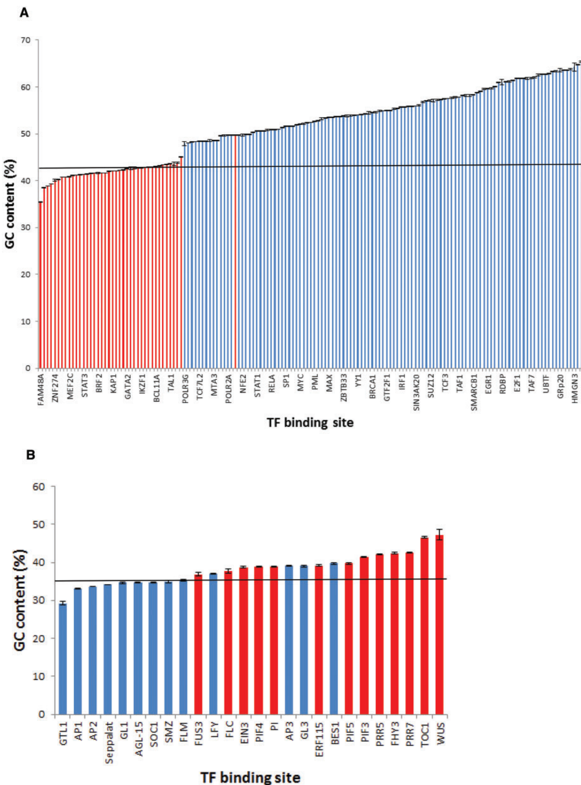
Fig. 7. —The GC content distribution for vertebrate and plant TF binding sites. (A) The GC content distribution for vertebrate (human) TF binding sites. The ubiquitous binding sites are shown in blue bars and tissue specific binding sites are represented in red color. The black horizontal line represents the non-coding genomic GC content for human genome (43.3%). (B) GC content distribution for plant ( A. thaliana ) TF binding sites. Ubiquitous binding sites are presented in blue color bars, whereas the tissue specific binding sites are provided in red color. The black horizontal line represents the non-coding genomic GC content for Arabidopsis genome (35.6%).
