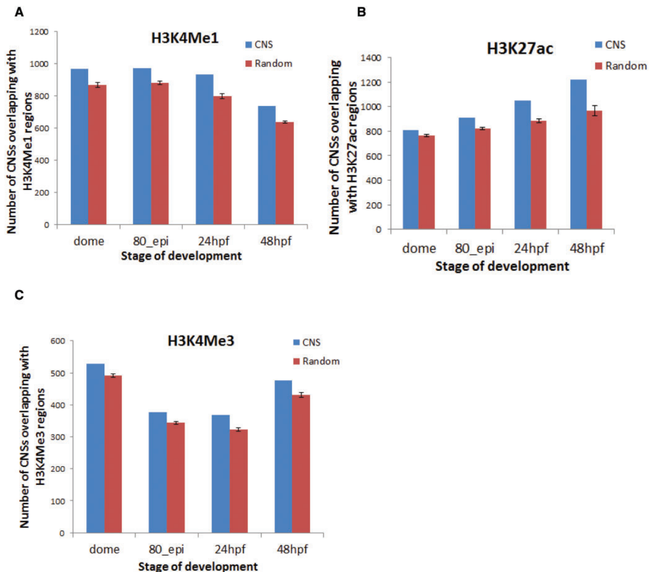
Fig. 5. —Chromatin modification signals overlapping with teleost fish CNSs at different development stages. (A) CNSs overlapping with H3K4Me1 regions. (B) CNSs overlapping with H3K27ac regions. (C) CNSs overlapping with H3K4Me3 regions. The statistical significance of the number CNSs overlapping with chromatin modification signals was compared with random samples overlapping chromatin modification signals with t -test at 95% confidence.
