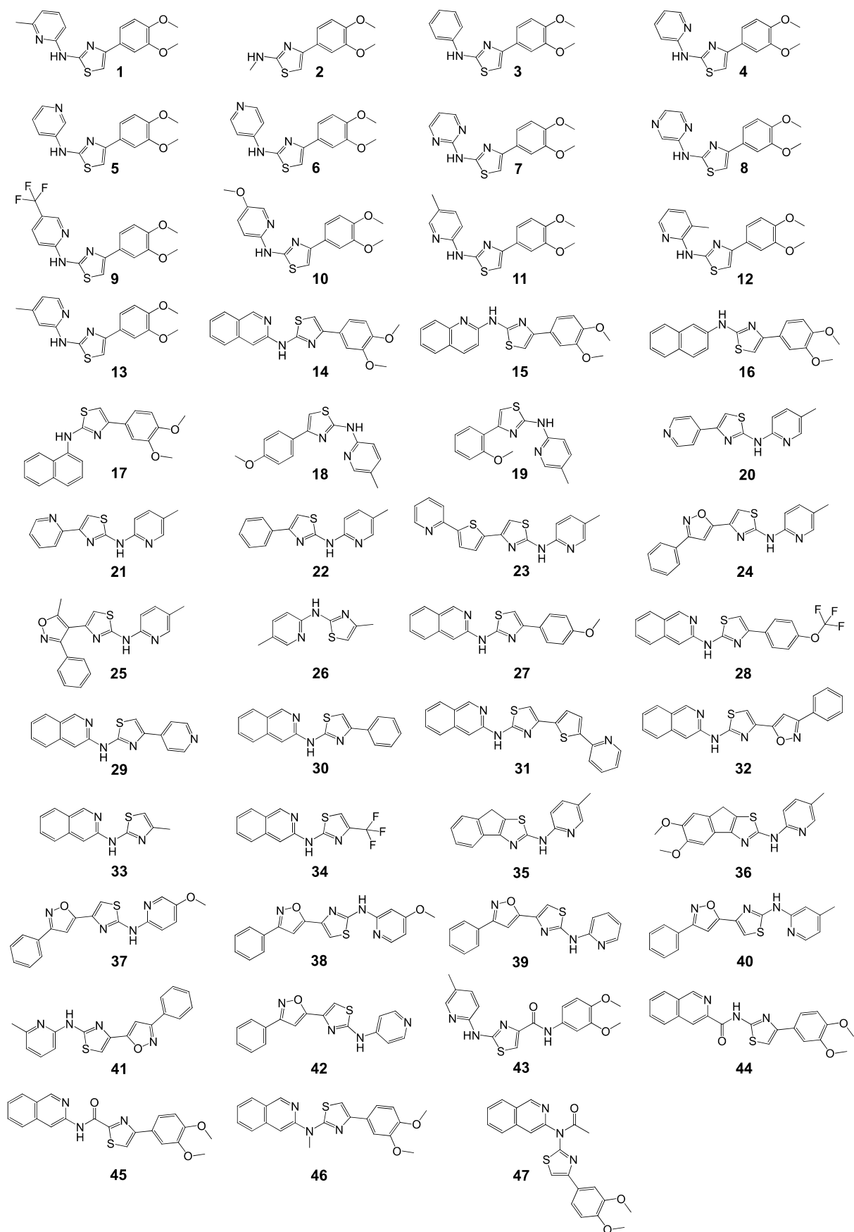
Figure 1: Chemical structure of 2-aminothiazole derivatives
