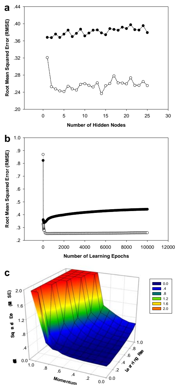
Figure 3: Optimization of ANN parameters comprising of the number of hidden nodes (a), the number of learning epochs (b) and the learning rate and momentum
