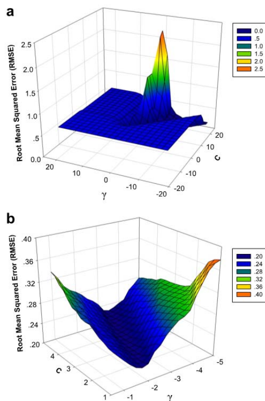
Figure 2: Optimization of SVM parameters comprising of an initial coarse grid search (a) and local grid search (b)
