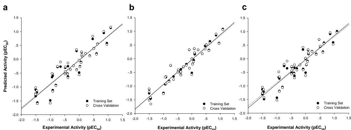
Figure 4: Plot of the experimental versus predicted values of pEC_{50} as obtained from MLR (a), SVM (b), and ANN (c) calculations
