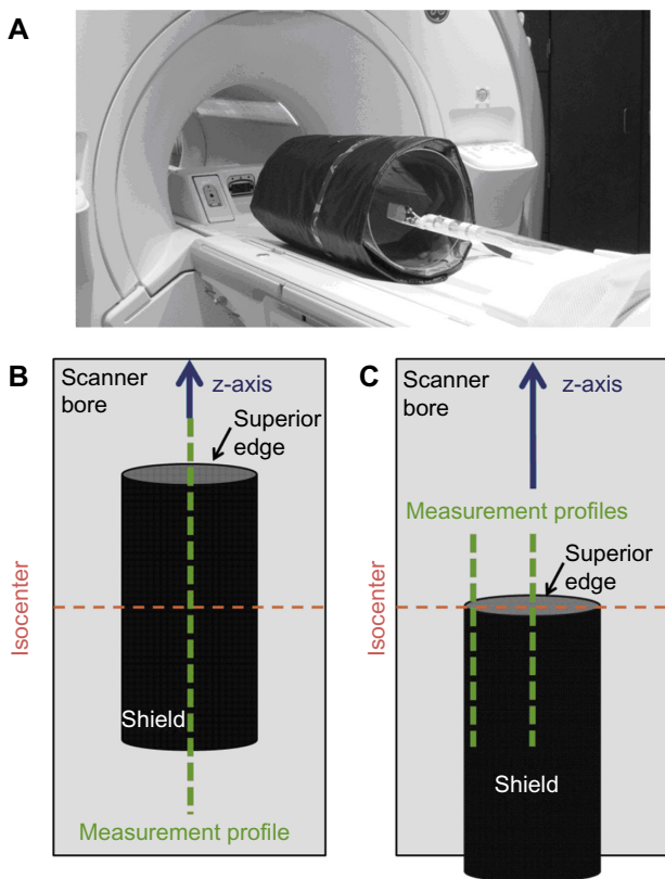
Figure 1 Experimental setup for direct measurements of RF attenuation. Notes: (A) Photograph of the set-up. The RF shield (wrapped around acrylic cylinder) was positioned within the bore of the 1.5 T and 3.0 T scanners. (B) Experimental configuration utilized to measure the RF attenuation of the shield. (C) Experiment configuration utilized to measure the RF field outside of the shield. In both (B and C), the dashed green lines represent the lines along which measurements were acquired.
