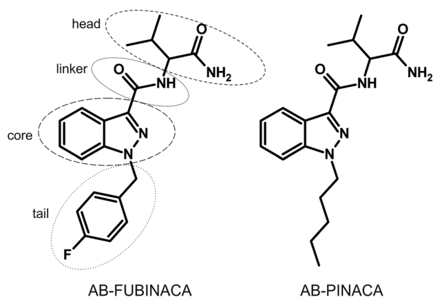
Fig. 1 Chemical structures of AB-FUBINACA and AB-PINACA and indication of the four subunits in the structure of synthetic cannabinoids
