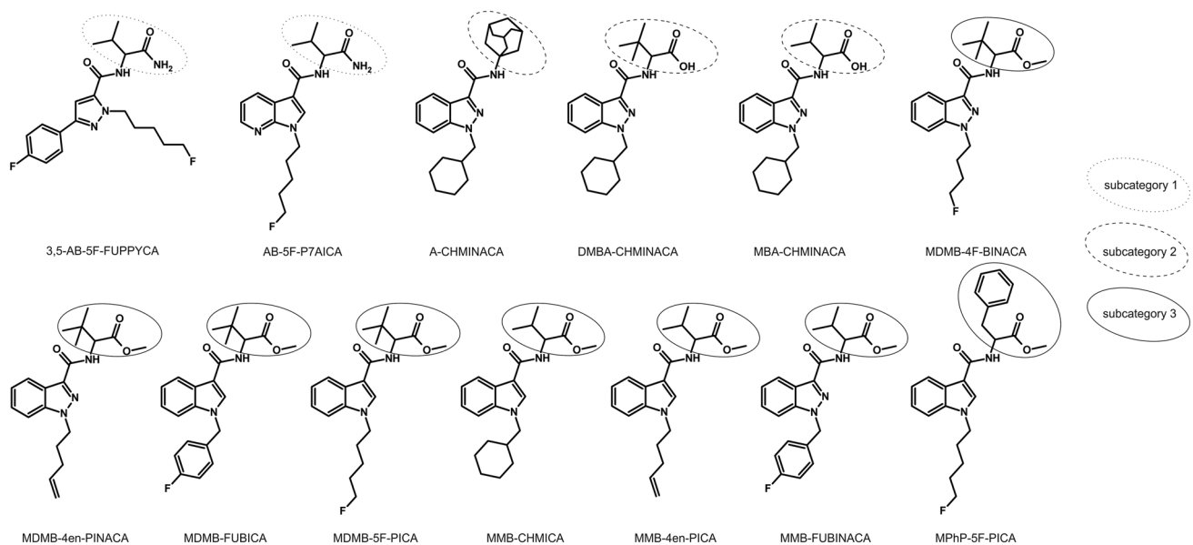
Fig. 2 Chemical structures of the 13 tested synthetic cannabinoids including subcategory classification
