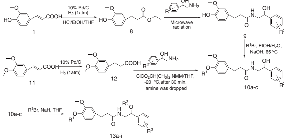
Scheme 2 Synthesis of hydrogenated ferulic acid amide derivatives 13.
