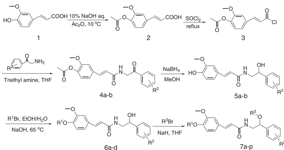
Scheme 1 Synthesis of ferulic acid amide derivatives 7.
