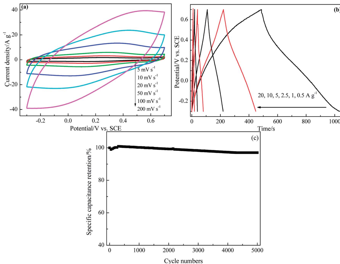
Fig. 5 Electrochemical capacitive properties of PRGF-0.75 electrode measured using a three-electrode system in 0.5 mol \text{L}^{-1} \text{H}_2\text{SO}_4 electrolyte: (a) CV curves at different scan rates. (b) Galvanostatic charge/discharge profiles at different current densities. (c) Cycle stability at a current density of 5 \text{A g}^{-1} .
