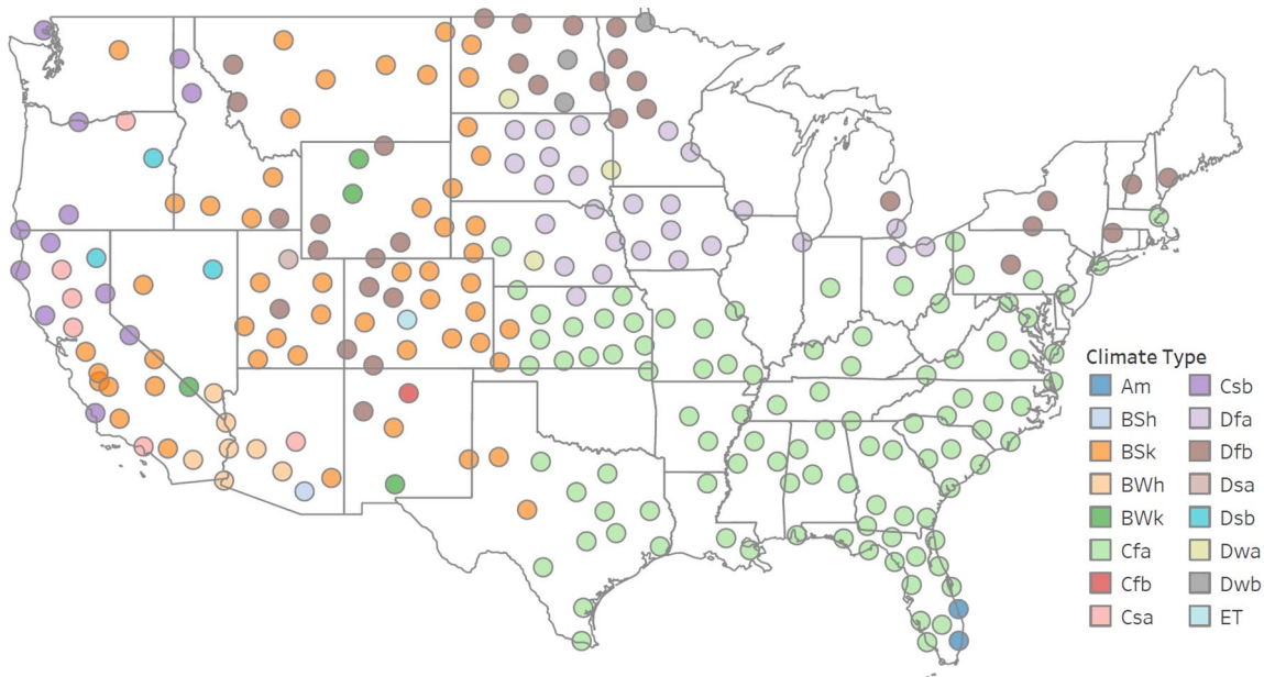
Figure 2. Spatial distributions of in-situ stations based on Köppen climates according to Table 1.
