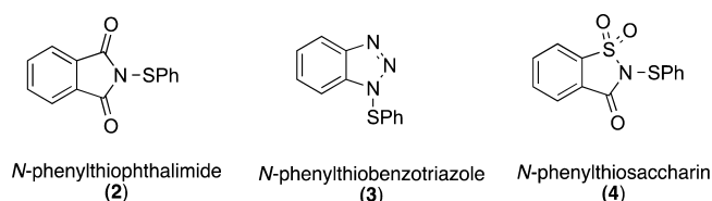
Figure 1. Sulfenylating agents.
