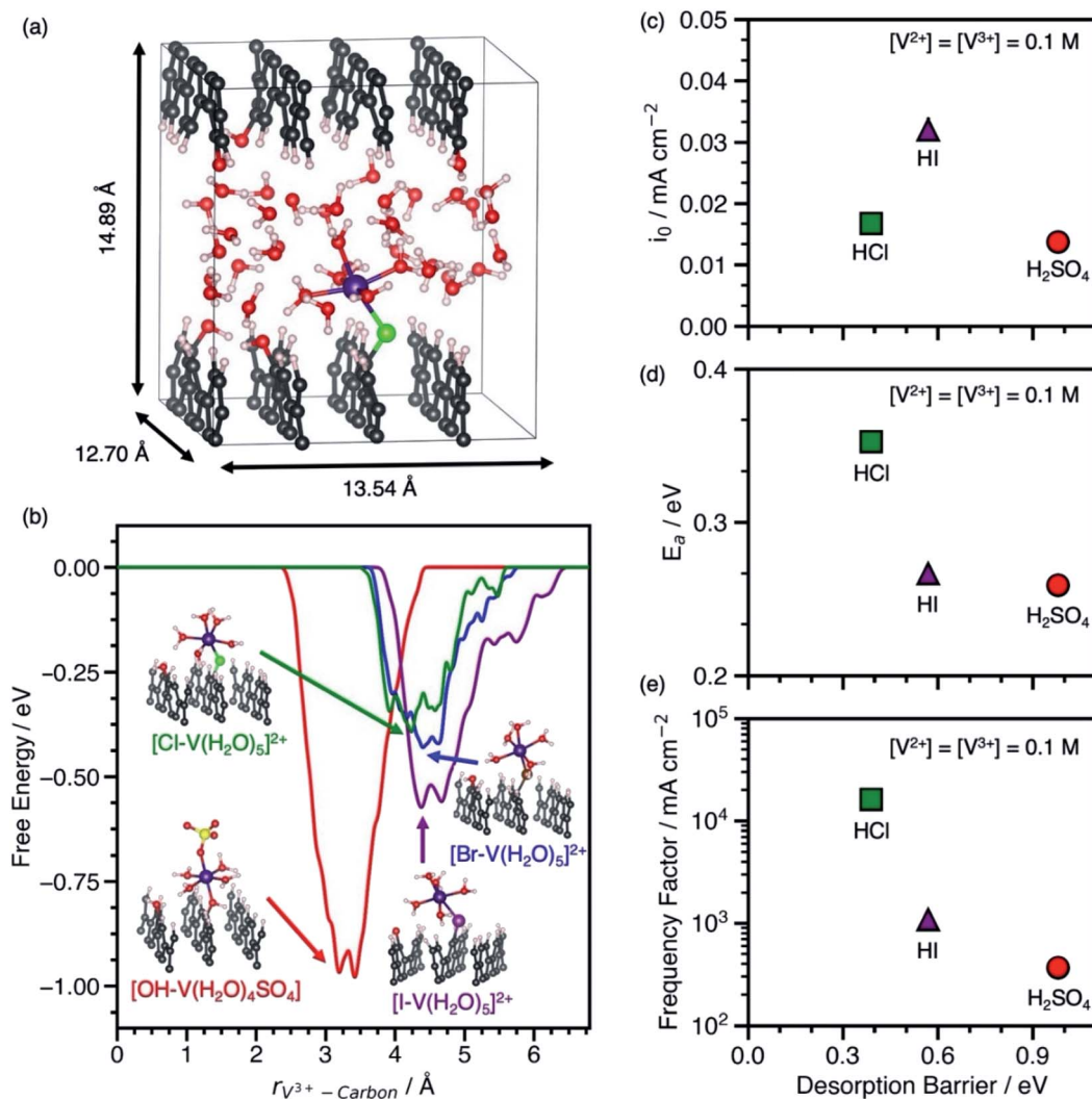
Fig. 2 (a) Cell used for metadynamics simulations of V 3+ -anion complexes on graphite(1120). (b) Free energy vs. the distance between the V 3+ ion and the carbon surface for V 3+ -anion complexes adsorbed to graphite(1120) through an *OH, *Cl, *Br, or *I bridge at 300 K. Geometries of adsorbed V 3+ -anion complexes at the free energy minima are shown next to the corresponding free energy profile in H 2 SO 4 (red line), HCl (green line), HBr (blue line), and HI (purple line). Atom color legend: C = gray, V = violet, O = red, S = yellow, H = white, Cl = green, Br = dark brown, I = purple. (c) V 2+ /V 3+ exchange current density ( i 0 ) at room temperature (T = 23.3 °C) on EPPG in H 2 SO 4 , HCl, and HI from steady-state current densities as a function of voltage extrapolated to equilibrium voltage using the Tafel equation vs. the V 3+ -anion complex desorption barrier. (d) V 2+ /V 3+ apparent activation energy ( E a ) in H 2 SO 4 , HCl, and HI extracted from the temperature dependence of i 0 from measurements between 23.3–40 °C vs. the V 3+ -anion complex desorption barrier. (e) V 2+ /V 3+ frequency factors vs. the V 3+ -anion complex desorption barrier. For all experimental measurements in (c–e), the acid concentration is 1 M and concentrations of both V 2+ and V 3+ are 0.1 M.
