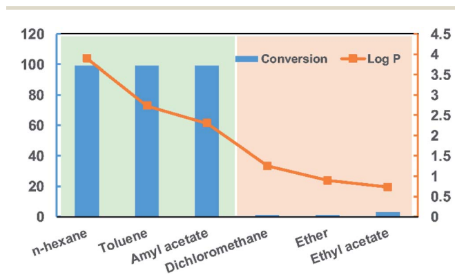
Fig. 2 Effect of organic solvents in biphasic reaction system on the dehydration of BAOx to BN by OxdF1. \log P values are plotted to correlate enzyme activity with the hydrophobicity of the organic solvents.
