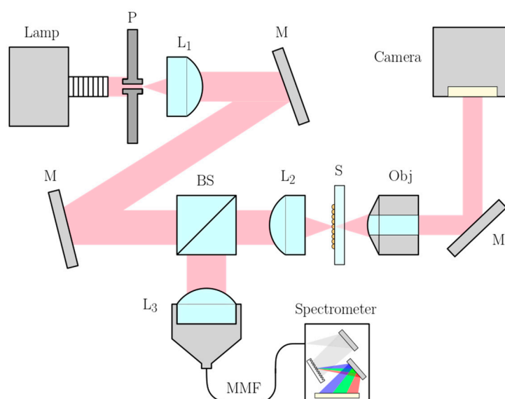
Figure 1. Optical reflectance and transmittance measurement setup: P: pinhole, L: lens, M: mirror, BS: beamsplitter, S: sample, Obj: microscope objective, MMF: multimode fiber.
