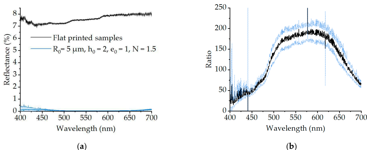
Figure 4. Effect of the printed geometries on the reflectance spectra. (a) Average reflectance spectra of the flat printed samples and of the optimized microlens array sample, with respective error of 1\sigma ; (b) Ratio between the flat and optimized structure's reflectance with blue lines showing error of 1\sigma .
