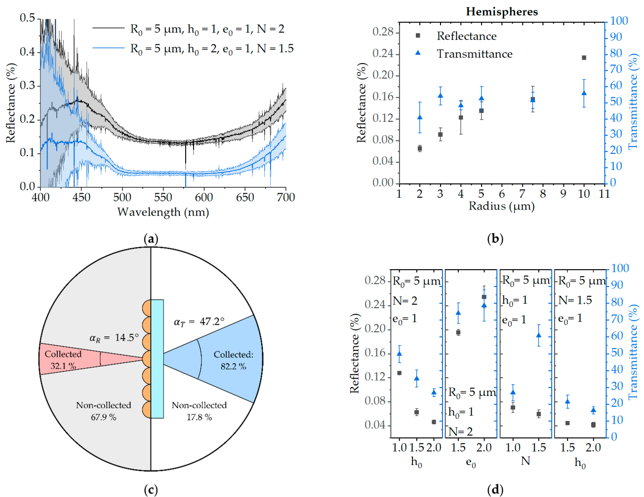
Figure 3. Structure's reflectance and transmittance characteristics as a function of the design parameter from Equation (1). (a) Reflectance spectra of the most and least reflective structures with error and corresponding shape parameters; (b,d) average reflectance (at \lambda = 550 \text{ nm} ) and transmittance of structures printed with corresponding error: (b) Hemispheres with varying radius R_0 ( h_0 = 1, e_0 = 1 and N = 2 ), (d) structures with varying height factor, h_0 , elongation factor, e_0 , pyramidal factor, N , and combinations of these parameters; (c) Collection angles and percentage of collected and transmitted light intensity estimation based on calculation in Section S5 (for a hemisphere with R_0 = 5 \mu\text{m} and at \lambda = 550 \text{ nm} ). All errors in (a,b,d) correspond to 1\sigma .
