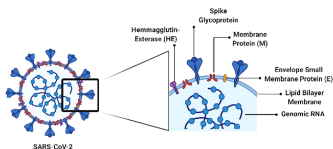
Figure 1. Cartoon representation of SARS-CoV-2 viral structure. Figure made in Biorender.
