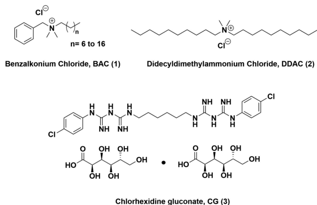
Figure 2. Chemical structures of QACs reviewed in ref 15.
