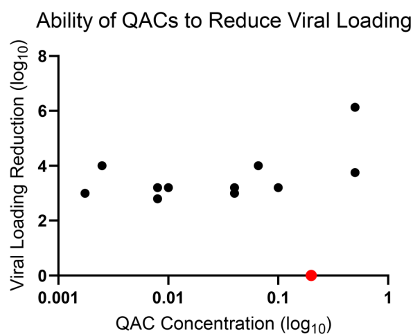
Figure 4. Graph displaying reduction in viral load by various QACs. Data were obtained from Table 1. Note that QAC concentration is displayed in \log_{10} for clarity. Data points that are listed as viral load reduction of >3.0 or <3.0 were given values of 3.2 and 2.8, respectively, to aid in clarity. Additionally, data from Ansaldi et al. were omitted as it did not contain viral load reduction values. An outlier from a data set (Wood et al. 19 ) used for CDC reference is marked in red.
