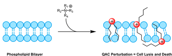
Figure 3. Mode of action of QACs against both bacterial and viral phospholipid membranes. Red spheres represent positively charged nitrogen atoms.
