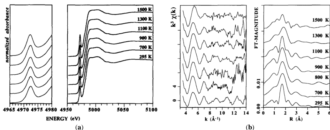
Figure 17. (a) Pre-edge (left) and XANES spectra (right) collected at Ti K-edge of NTS2 ( 46.1\text{SiO}_2-0.07\text{K}_2\text{O}-24.0\text{Na}_2\text{O}-30.6\text{TiO}_2 wt %) glass and melt; (b) Normalized k^3 weighted EXAFS spectra (left) and Fourier Transform (right) of the same glass [52]. “Reproduced with permission from published by © Elsevier.” (2017).
