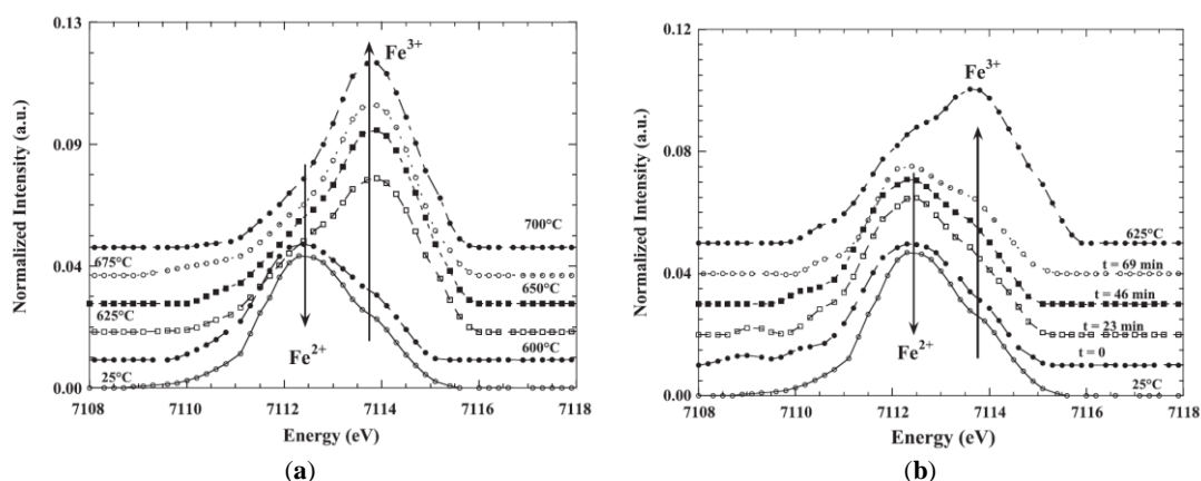
Figure 18. Evolution of the Fe K-edge pre-edge peak with temperature and time for PyrNa17R glass ( 52.98\text{SiO}_2-11.99\text{MgO}-17.00\text{CaO}-5.48\text{Na}_2\text{O}-12.75\text{FeO} ): (a) collected at different temperatures; (b) collected at 600 °C at different times in comparison with the pre-edge data collected at 25 °C and 625 °C [59]. “Reproduced with permission from published by © Elsevier.” (2017).
