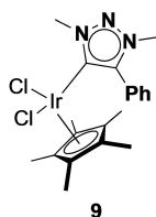
Figure 1. Structure of simple triazolylidene complex 9 .
