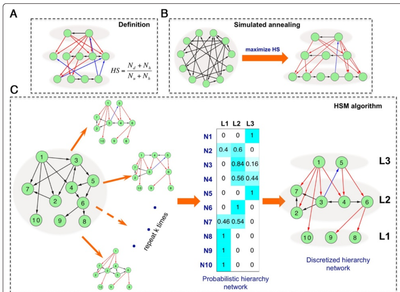
Figure 1 The schematic diagram of the hierarchy score maximization algorithm. In hierarchical networks, the downward, upward, and horizontal edges are shown in red, blue, and black colors, respectively. (A) The definition of hierarchy score. (B) A simulated annealing algorithm for inferring the hierarchical structure by maximizing the hierarchy score. (C) The procedure to calculate the probability of nodes in different hierarchy levels. Simulated annealing procedure is performed for k runs and in each run a hierarchical structure is inferred by maximizing the hierarchy score. The frequency of each node in these k hierarchical networks is calculated to obtain a probabilistic hierarchical network. Discretized hierarchical network is obtained by assigning nodes to the level with highest frequency.
