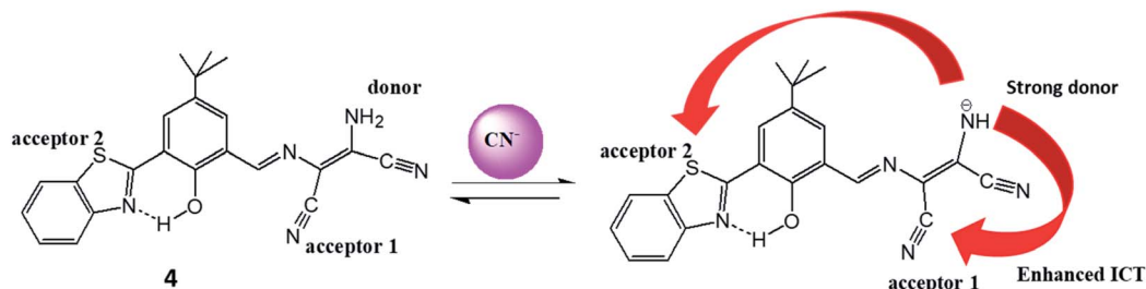
Fig. 6 The mechanism for the fluorescence response of sensor (4) to \text{CN}^- ion.
