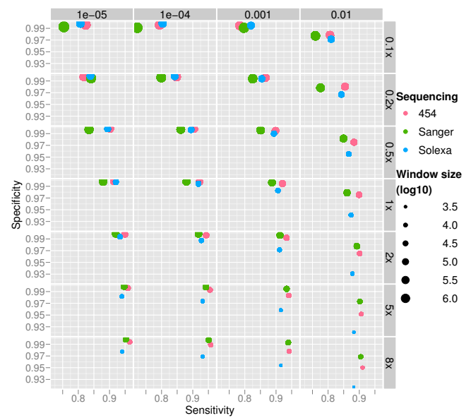
Figure 3 Performance of CNV-seq. The performance of CNV-seq on data simulating 454, Sanger and Solexa methods. Results are shown for 0.1\times – 8\times coverages (right) and p -value range of 10^{-5} – 10^{-2} (top). Each dot represents an average of 100 simulations and the size of the dots represents the window ( \log_{10} ) size, i.e. resolution used. The window sizes are calculated using equation (5).
