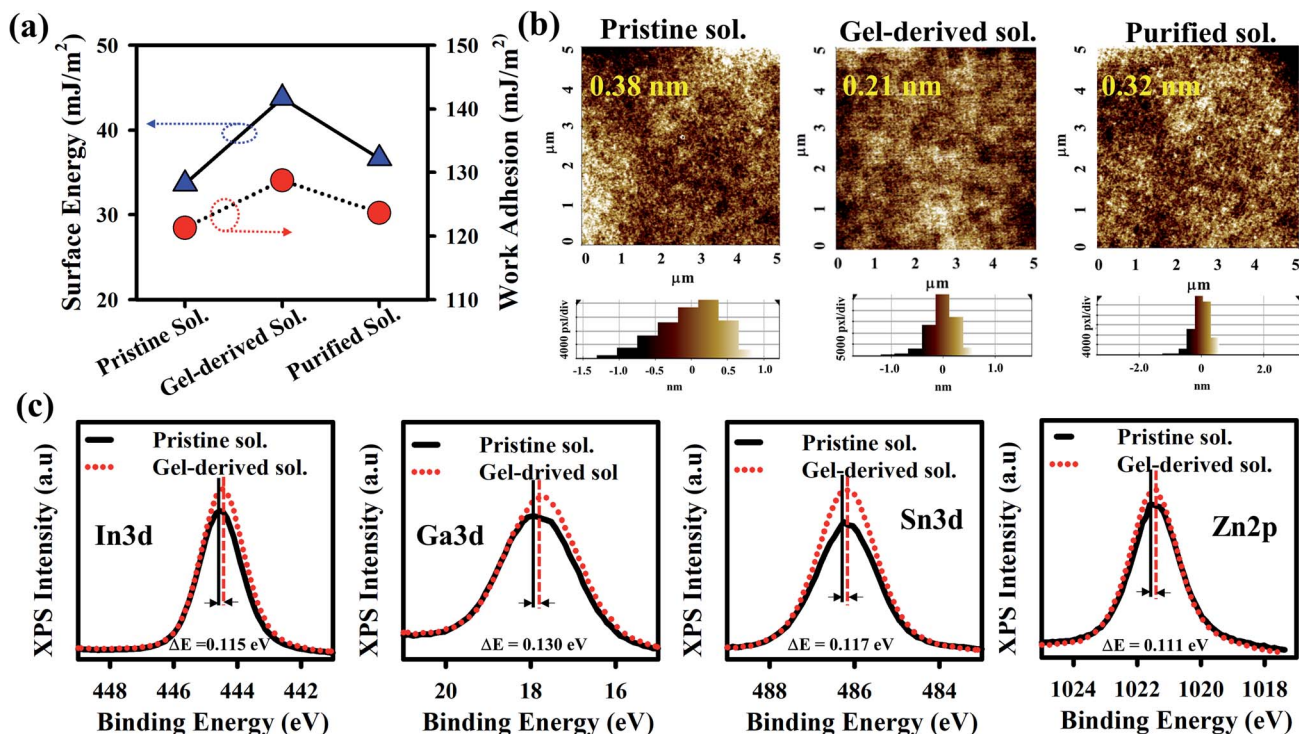
Fig. 2 Surface morphology and chemical bonding analysis of the GITZO films. (a) Surface energy and work adhesion for the pristine, gel-derived, and purified GITZO films. (b) AFM image (scan size: 5 μm × 5 μm) of three GITZO thin films. The RMS roughness of the GITZO film is lower for the gel-derived precursor material. The smooth surface of the film by gel-derived precursor provides more electron-conducting pathways and reduces the trap density. (c) XPS core-level spectra of In 3d 5 , Ga 3d, Zn 2p 3 , and Sn 3d 5 , obtained from the GITZO thin films. Their respective peak intensities increase in the gel-derived film. All cation binding energy peaks shift to the lower binding energy, indicating the reduction of oxygen-related defects for the gel-derived GITZO.
