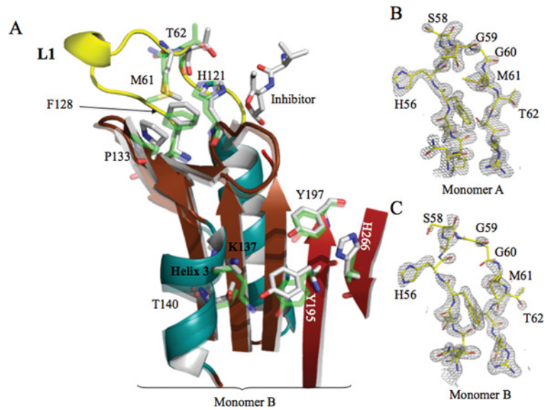
Figure 2 Comparison of changes resulting from the Val 266 to histidine mutation (A) Conformational changes in the dimer interface, helix 3 and active site of the V266H variant compared with wild-type caspase 3. The wild-type protein is shown as partially transparent secondary structure with amino acid side chains in green. The electron density maps of loop 1 from monomer A (B) or monomer B (C) show disorder in L1 of monomer B.
