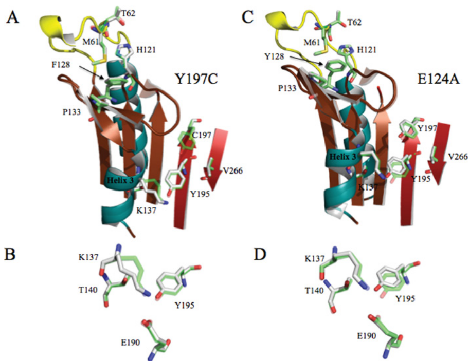
Figure S5 Comparison of single mutants Y197C (A, B) or E124A (C, D) with wild-type caspase 3 (A–D) Wild-type caspase 3 is shown as partially transparent and amino acid side chains are coloured green. Amino acid side-chains for the mutants are coloured grey.
