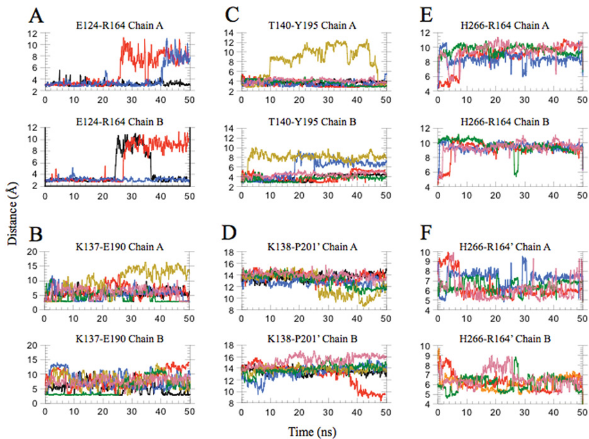
Figure S11 Distances were calculated for atom pairs over the course of the molecular dynamics simulation
