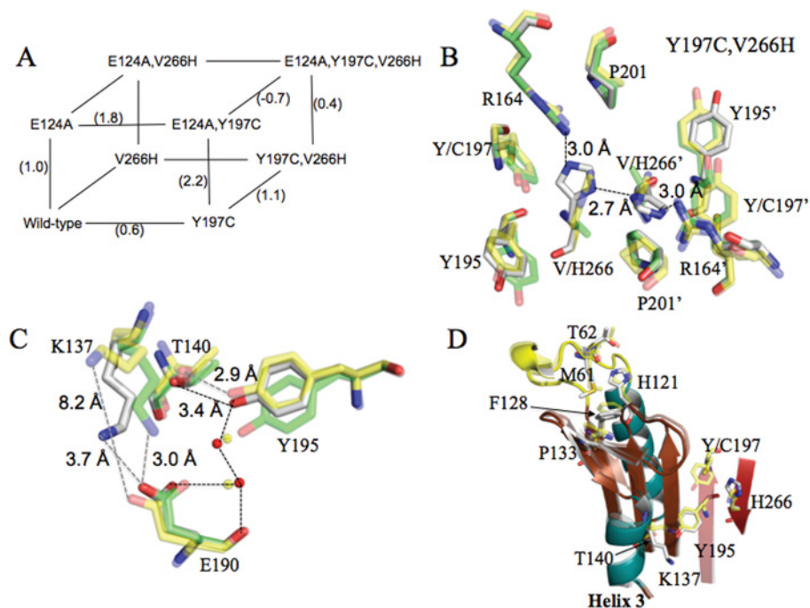
Figure 3 A double mutation of Y197C, V266H restores activity and structure similar to that of wild-type (A) Additional mutations made in the context of V266H. Numbers in parentheses indicate change in k_{cat}/K_m values in terms of \Delta\Delta G^\circ (kcal/mol), as described in the text. (B) Dimer interface of caspase-3 (Y197C, V266H). (C) Interactions among Lys 137 , Thr 140 , Glu 190 and Tyr 195 . (D) Comparison of changes in helix 3 and the active site of monomer B. For (B–D), the following colour scheme is used: Y197C, V266H (grey), V266H (yellow) and wild-type (green).
