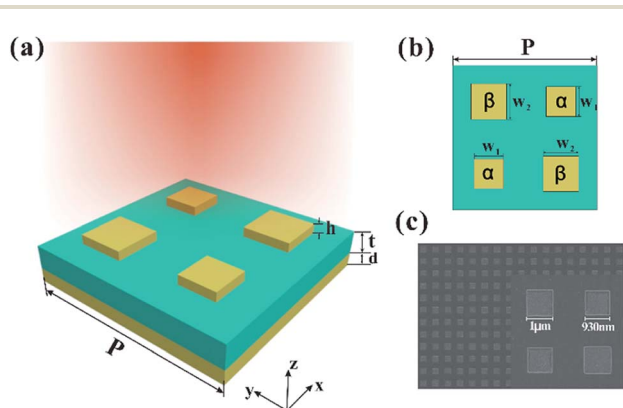
Fig. 1 (a) Schematic of the fabricated tunable broadband metamaterial absorber incorporating phase-change material GST. The thickness of top metal square, GST spacer and bottom Au mirror are h = 80 \text{ nm} , t = 250 \text{ nm} and d = 100 \text{ nm} , respectively. (b) Top view of the unit cell, the geometrical parameters are p = 4.4 \mu\text{m} , w_1 = 0.93 \mu\text{m} , w_2 = 1 \mu\text{m} . (c) SEM image of the fabricated sample.
