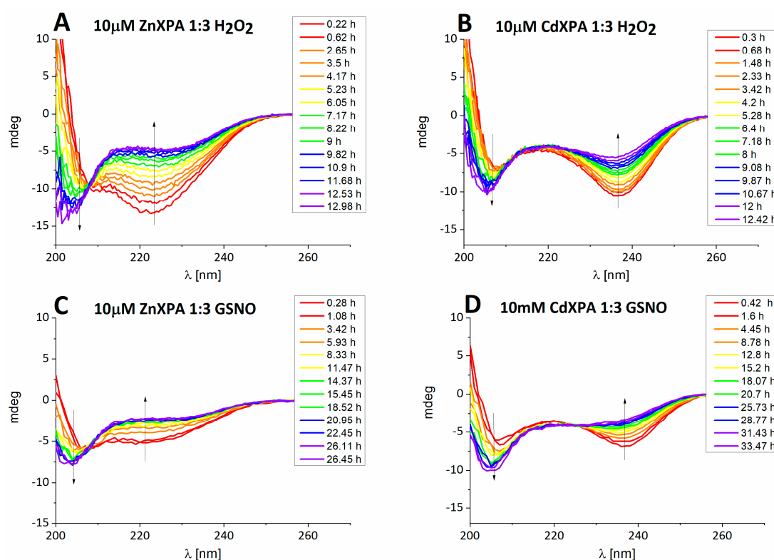
Figure 1. Examples of the time course of 10 \mu\text{M} ZnXPAzf and CdXPAzf decomposition by 3-fold molar excess of \text{H}_2\text{O}_2 or GSNO in 10 mM ammonium acetate buffer, pH 7.4, followed by CD spectroscopy. (A) ZnXPAzf and \text{H}_2\text{O}_2 ; (B) CdXPAzf and \text{H}_2\text{O}_2 ; (C) ZnXPAzf and GSNO; (D) CdXPAzf and GSNO. The time points (hours) are indicated in the graph.
