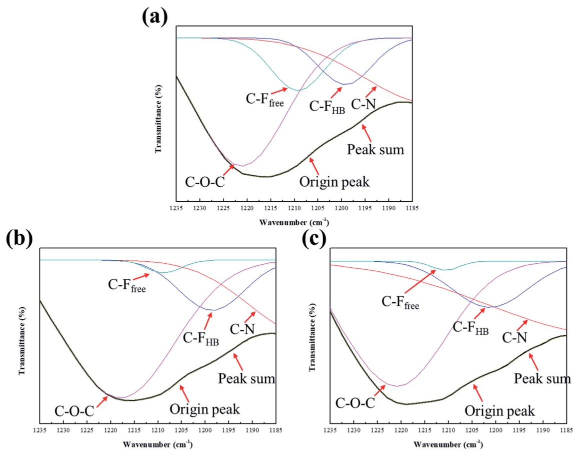
Fig. 6 FT-IR spectra of (a) 8FCOPU; (b) 12FCOPU; (c) 16FCOPU at the wavenumber range of 1235–1185 cm -1 .
