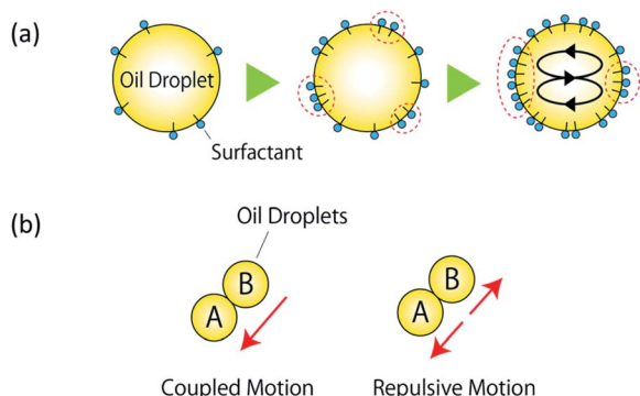
Fig. 1 Model of self-propelled oil droplets. (a) Driving force; (b) correlated motion.
