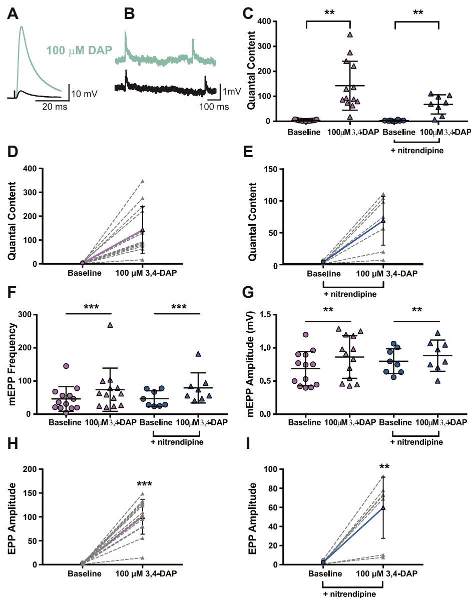
Figure 8. 100- \mu M 3,4-DAP dose dependently increases neuromuscular transmission independent of Cav1 channels in frog neuromuscular junctions. A and B, sample traces of electrophysiological recordings of EPPs (A) and mEPPs (B) before and after 100- \mu M 3,4-DAP application. C, quantified quantal content before (circles) or after (triangles) 100- \mu M 3,4-DAP application to vehicle (pink) or nitrendipine (blue) treated frog NMJs. Two-way mixed ANOVA was used (there was a significant main effect of 100- \mu M 3,4-DAP ( F(1, 19) = 31.66 , ***p < 0.0001 ); no significant main effect of nitrendipine ( F(1, 19) = 4.226 , p = 0.0538 ) nor a significant interaction between 3,4-DAP x nitrendipine ( F(1, 19) = 4.162 , p = 0.0555 ); vehicle, n = 13 ; nitrendipine n = 8 ). D and E, plots of individual paired values (gray dotted lines) with a superimposed average (solid pink line, vehicle; solid blue line, nitrendipine). F, the 100- \mu M dose of 3,4-DAP increased mEPP frequency in both the vehicle (pink) and nitrendipine (blue) conditions; two-way mixed ANOVA (significant main effect of 3,4-DAP; F(1, 19) = 9.541 , p = 0.006 ; no main effect of nitrendipine; F(1, 19) = 0.0264 , p = 0.8727 ) or a significant interaction between 3,4-DAP and nitrendipine; F(1, 19) = 0.0568 , p = 0.8143 ). G, the 100- \mu M dose of 3,4-DAP significantly altered mEPP amplitude in both the vehicle (pink) and nitrendipine (blue) conditions; two-way mixed ANOVA (significant main effect of 3,4-DAP; F(1, 19) = 11.88 , p = 0.0027 , but not nitrendipine; F(1, 19) = 0.3468 , p = 0.5628 , and no significant interaction between 3,4-DAP and nitrendipine; F(1, 19) = 1.436 , p = 0.2454 ). H and I, the 100- \mu M dose of 3,4-DAP increased EPP amplitude, shown as individual pairs (gray dotted lines) with a superimposed average (solid pink line, vehicle; H; solid blue line, nitrendipine, I); paired t test, **p = 0.0012 , ***p < 0.0001 . 3,4-DAP, 3,4-diaminopyridine; Cav, voltage-gated calcium; EPP, endplate potential; mEPP, miniature EPPs; NMJ, neuromuscular junction.
