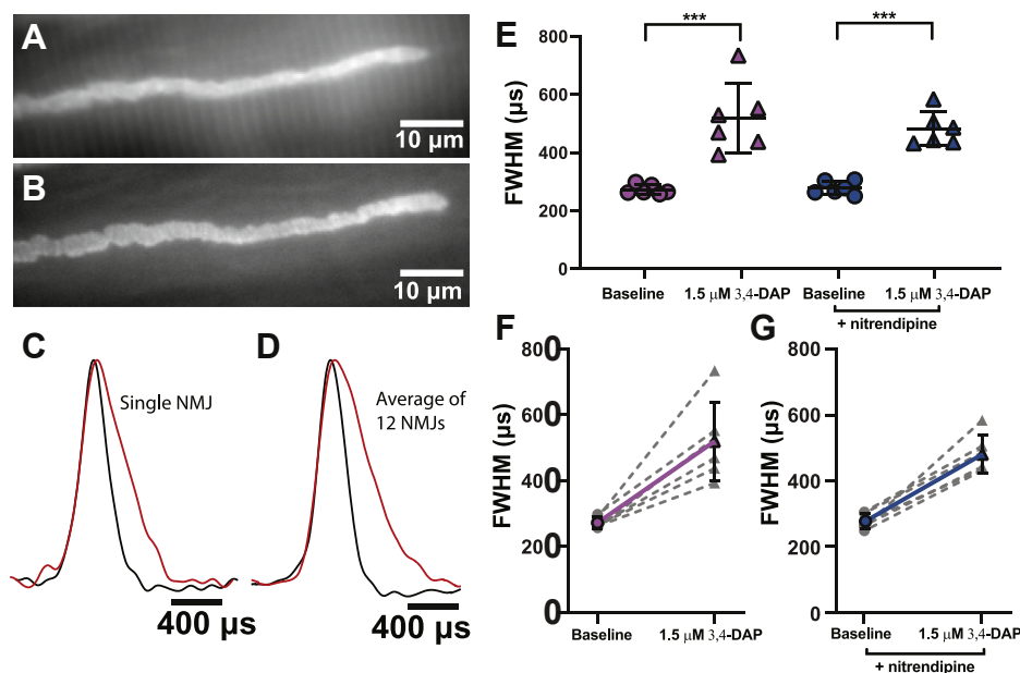
Figure 3. Therapeutic concentrations of 3,4-DAP broaden the presynaptic AP waveform independent of Cav 1 channels at the frog NMJ. A, a BeRS1 dye-stained image of a frog presynaptic motor nerve terminal. B, an Alexa Fluor 488 BTX-stained image of the same terminal as in A. C, normalized presynaptic AP waveform splines recorded from a single nerve terminal before (black) and after (red) the addition of 1.5- \mu M 3,4-DAP. D, the normalized average of all pre-drug (black) and post-1.5- \mu M 3,4-DAP (red) presynaptic AP waveform splines recorded from all frog motor nerve terminals ( n = 12 ). E, FWHMs of recorded AP waveforms before (circles) or after (triangles) 1.5- \mu M 3,4-DAP application to vehicle (pink) or nitrendipine (blue) treated frog NMJs. 1.5 \mu M 3,4-DAP broadens the AP waveform independent of nitrendipine (two-way mixed ANOVA: there was a significant main effect of 1.5- \mu M 3,4-DAP ( F(1,10) = 77.68 , ***p < 0.0001 ), but no main effect of nitrendipine ( F(1,10) = 0.2967 , p = 0.5979 ), and no significant interaction between 1.5- \mu M 3,4-DAP and nitrendipine ( F(1,10) = 0.7278 , p = 0.4136 ); vehicle, n = 6 ; nitrendipine, n = 6 ). F-G, plots of individual paired recorded values (gray dotted lines) of AP duration (FWHM) before and after application of 1.5- \mu M 3,4-DAP with a superimposed average (vehicle, solid pink line; nitrendipine, solid blue line). BTX, alpha-bungarotoxin; Cav, voltage-gated calcium; 3,4-DAP, 3,4-diaminopyridine; AP, action potential; BeRS1, Berkeley red-based sensor of transmembrane potential; FWHM, full width at half maximum; NMJ, neuromuscular junction.
