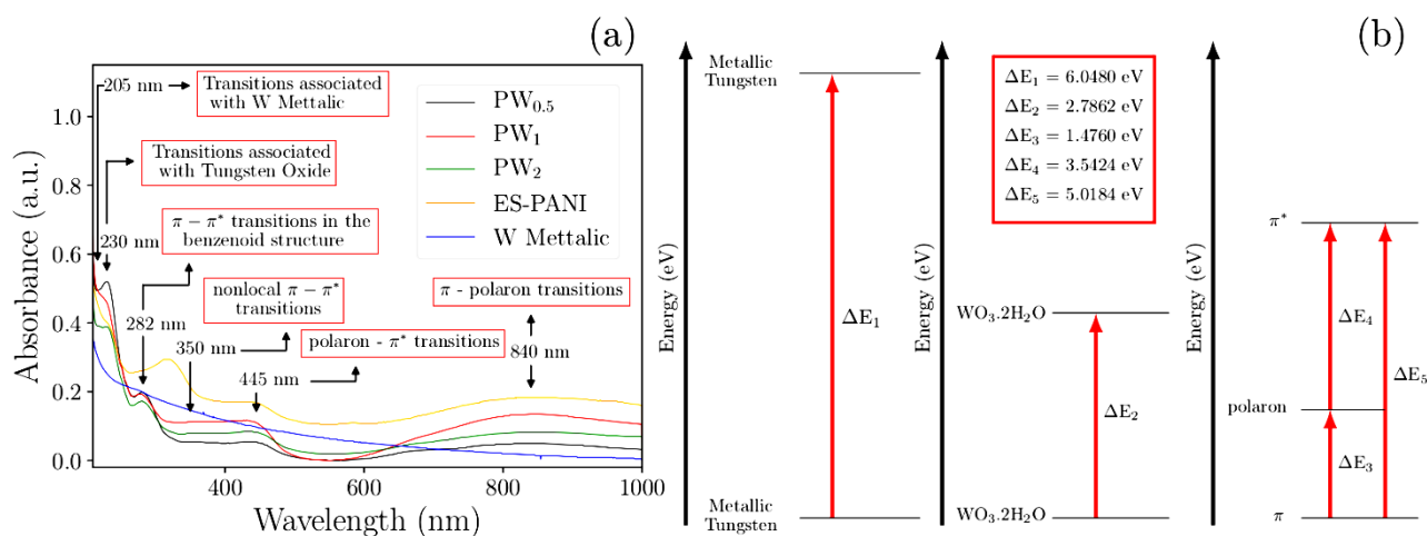
Figure 6. (a) UV-VIS spectra of the as -synthesized nanocomposites PW 0.5 , PW 1 and PW 2 showing the main polaronic state transitions, as well as the peaks related to the metallic W and WO 3 ·2H 2 O phases. (b) Schematic representation of the electronic transitions between phases.
