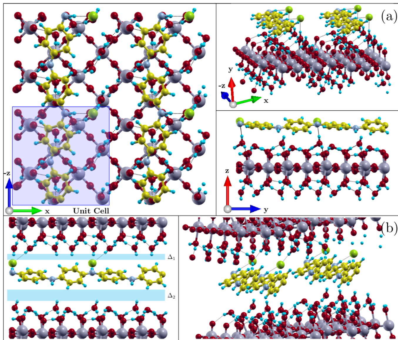
Figure 2. (a) Optimized structure of the periodically replicated PWO–CIS system (unit cell highlighted in blue). The polymeric phase was deposited on a \text{WO}_3 \cdot 2\text{H}_2\text{O} layer and, after geometric optimization, presented a distance of 0.60 Å. No changes in their molecular structures were observed, only a rearrangement in their bond lengths. (b) Optimized structure of the periodically replicated PWO–CIB system. The polymer phase interacted with two layers of \text{WO}_3 \cdot 2\text{H}_2\text{O} , presenting distances of \Delta_1 = 1.17 Å and \Delta_2 = 1.78 Å between the upper and bottom layers, respectively. No changes in their molecular structures were observed, only a rearrangement in their bond lengths in addition to the interaction between counter ions, polymer layer, and upper oxide layer.
