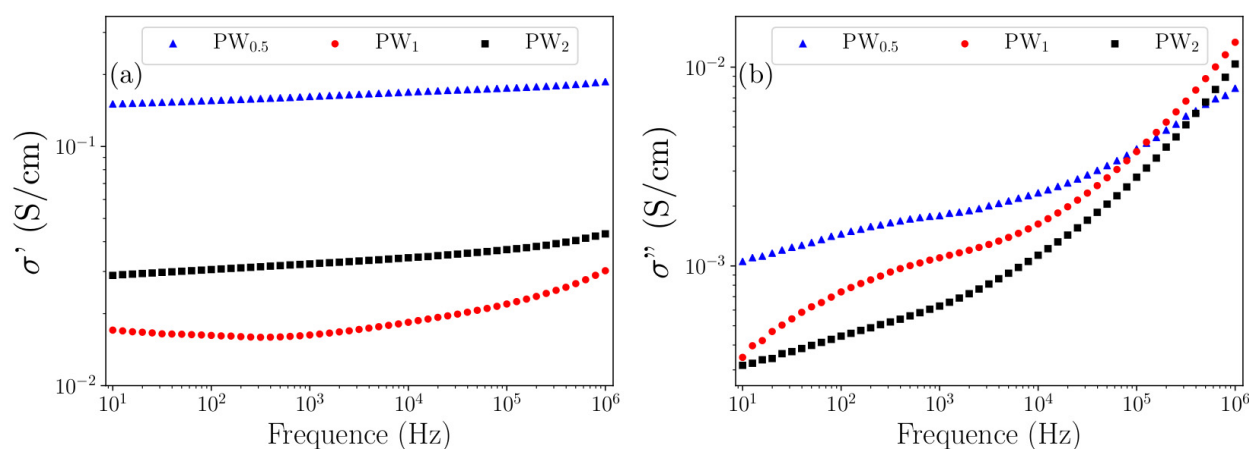
Figure 7. (a) Real and (b) Imaginary complex conductivity spectrum of nanocomposites.
