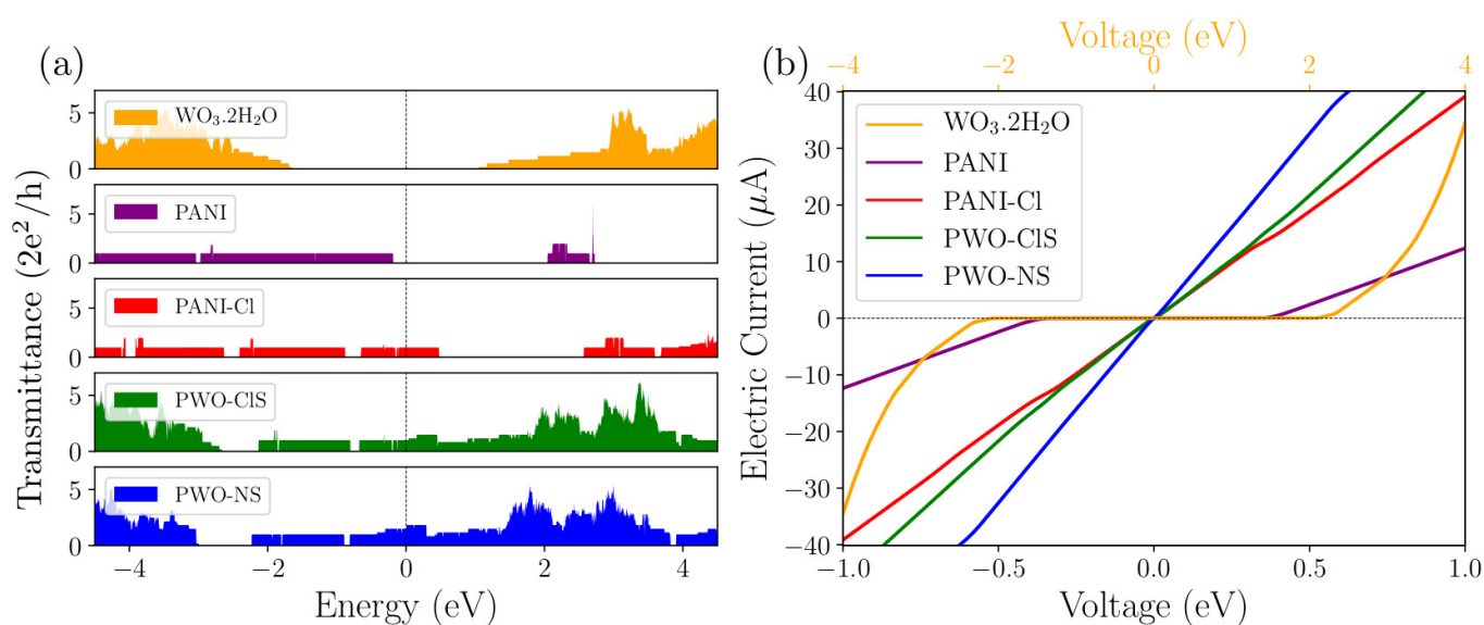
Figure 11. (a) Quantum transmittance spectrum of the proposed systems as a function of energy, considering E_F = 0 . The WO_3 \cdot 2H_2O and PANI models showed gap energy around the Fermi level of 2.6 eV and 2.2 eV, respectively. The other models presented conducting behavior in terms of electronic charge transport. (b) Electric current curves as a function of applied voltage for all proposed systems. The isolated systems WO_3 \cdot 2H_2O and PANI showed null electrical current in the ranges from 0.00 eV to 2.00 eV and from 0.00 eV to 0.37 eV, respectively, behaving as insulating materials. The doped PANI-Cl and the nanocomposite systems presented electrical current varying linearly as a function of the applied voltage, behaving as a metallic material.
