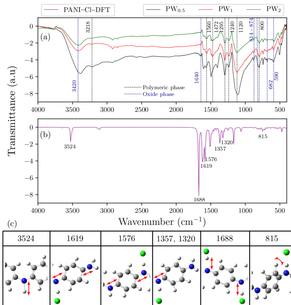
Figure 4. (a) Spectra of the as -synthesized PW_{0.5} , PW_1 and PW_2 nanocomposites showing the bands corresponding to the main vibrational modes. The bands resulting from the stretching and deformations of the polymeric phase were clearly identified; (b) Theoretical spectrum of ES-PANI and (c) Observed vibrational modes.
