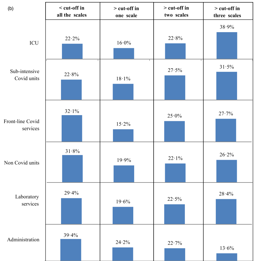
Fig. 1. a. Percentage of subjects reporting scores a) < the cut-off in the tree assessment measures; b) scores > cut-off in one assessment measure; c) scores > cut off in two assessment measures; d) scores > cut-off in all the three assessment measures by occupation. Figure 1b. Percentage of subjects reporting scores a) < the cut-off in the tree assessment measures; b) scores > cut-off in one assessment measure; c) scores > cut off in two assessment measures; d) scores > cut-off in all the three assessment measures by place of work.
