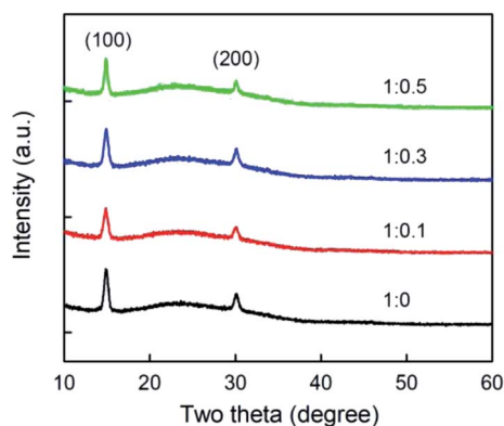
Fig. 3 XRD patterns of the \text{CH}_3\text{NH}_3\text{PbBr}_3 films on the PEDOT:PSS:GO films doped with different GO amount.
