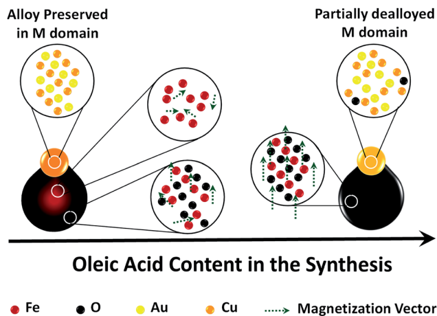
Scheme 2 Schematic summary of effect of changing the OlAc content in the synthesis.
