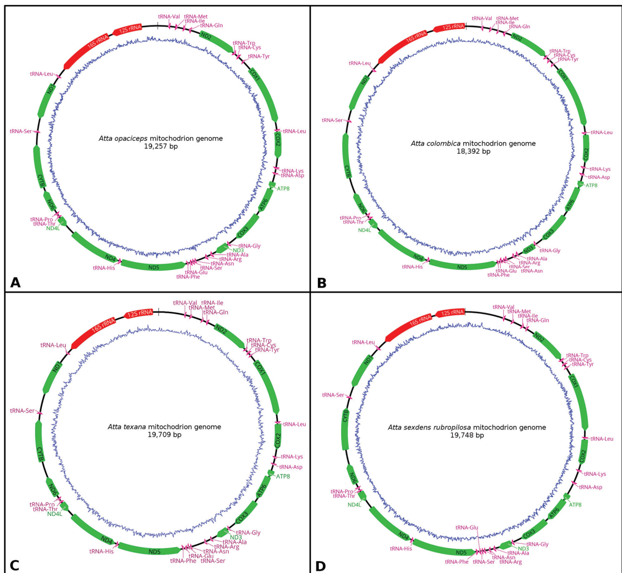
Figure 1 - Complete gene map of Atta opaciceps (A), Atta colombica (B), A. texana (C), and Atta sexdens rubropilosa (D) mitogenomes. Genes in the circle and outside the circle are transcribed in clockwise and counterclockwise directions, respectively. The protein-coding genes are shown in green, rRNAs in red, and tRNAs in purple. The green ring represents the A+T contents and the blue ring shows C+G contents.
