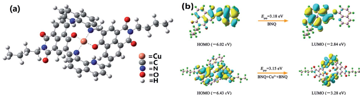
Fig. 5 (a) DFT optimised structures of \text{BNQ-Cu}^{2+}\text{-BNQ} complex. (b) Molecular orbital profiles of \text{BNQ} and \text{BNQ-Cu}^{2+}\text{-BNQ} molecules.
