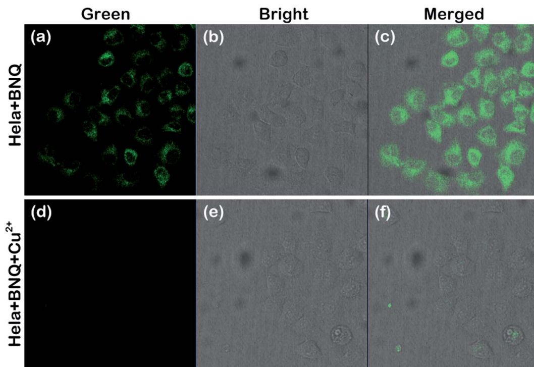
Fig. 6 Fluorescence images (a and d), bright-field transmission images (b and e) and merged images (c and f) of HeLa cells incubated with the \text{BNQ} probe (1 \mu\text{M} ) initially and 30 min after treatment with \text{Cu}^{2+} (10 \mu\text{M} , DMSO/HEPES = 1/9, v/v, pH = 6.0). \lambda_{\text{em}} = 515 \text{ nm} .
