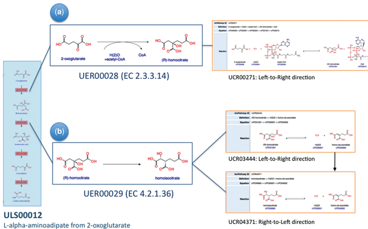
Figure 3. Example of relationships between ULS, UER and UCR. ULS00012—'L- \alpha -aminoadipate from 2-oxoglutarate'—is a linear subpathway composed of four UERs linked through their primary compounds. (a) The first step in ULS00012 is UER00028, associated to the chemical reaction UCR00271 (using Left-to-Right direction). This UCR involves five compounds, but only two of these, 2-oxoglutarate and (R)-homocitrate, are considered to be primary compounds in the context of UER00028. (b) The second step in ULS00012 is UER00029, associated to two chemical reactions: UCR03444 (using Left-to-Right direction) followed by UCR04371 (using Right-to-Left direction). The primary substrate of UER00029 is (R)-homocitrate and its primary product is homoisocitrate.
