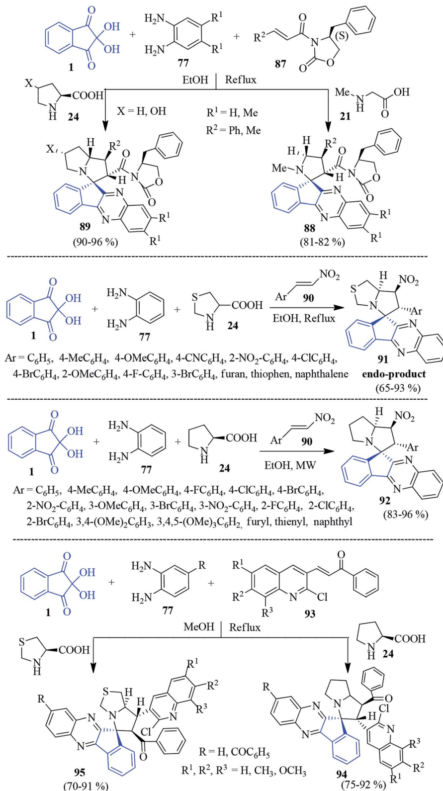
Scheme 30 Regioselective synthesis of spiro-indenoquinoxaline derivatives 88 , 89 , 91 , 92 , 94 , and 95 .
