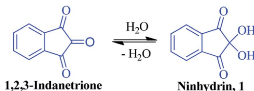
Fig. 1 Structure of ninhydrin.
