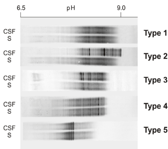
Figure 1. Isoelectric focussing on agarose gels with immunoblot: The figure represents the classical types 1 - 5 (Andersson et al. 1994):
