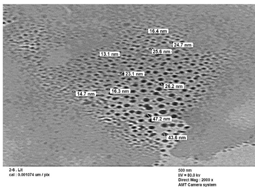
Figure 3 TEM image for selenium nanoparticles synthesized by using compound 2b at room temperature. Abbreviation: TEM, transmission electron microscope.
