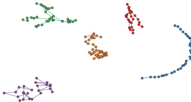
Fig. 5. Simulated trajectories: stop-and-go (green), flip directed (red), random (orange), fast random (purple) and curved directed (blue)
