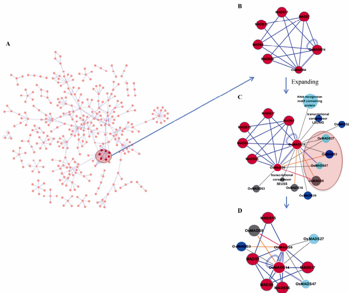
Figure 2 Expansion of MADS-box containing proteins. A. A small interactome network of rice with experimental identification visualized by Cytoscape. B. A functional motif constructed by seven MADS-box containing proteins in rice. C. An expanded sub-network of MADS-box related motif. Proteins in pink region are predicted as potential participants to the protein complex due to their tight interactions with the motif. D. A reconstructed sub-network with new participants.
