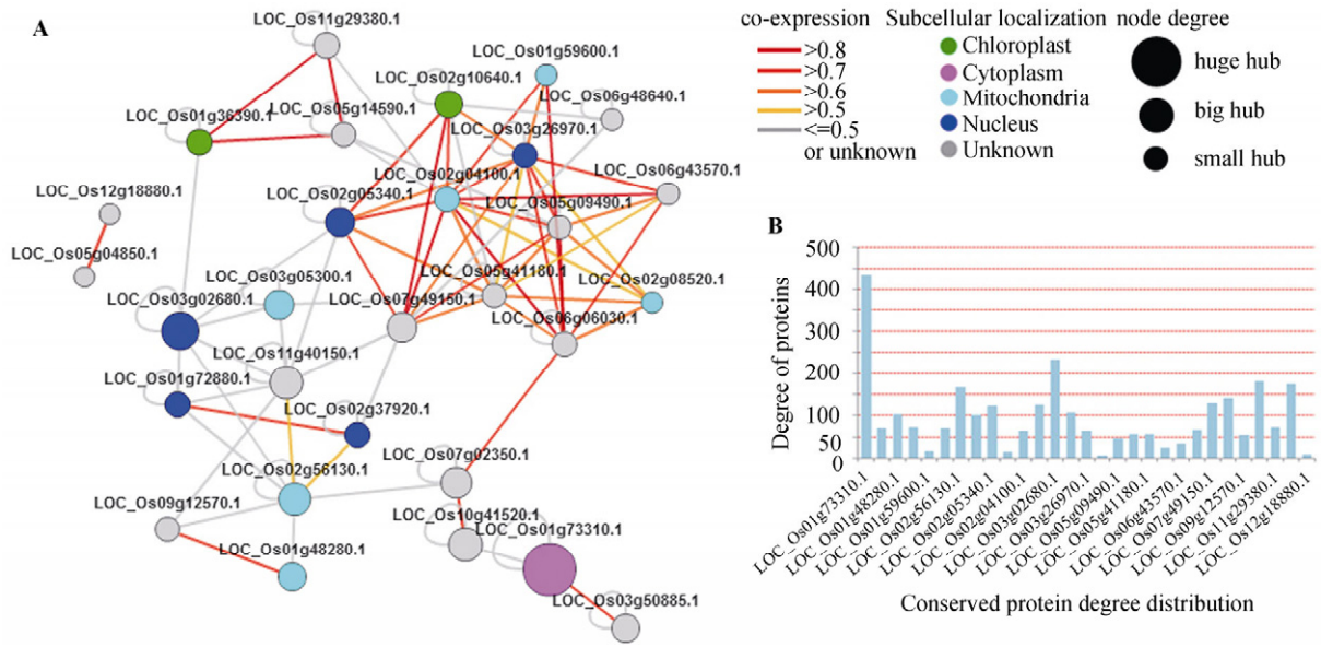
Figure 1 Evolutionarily conserved interaction sub-network. A . A sub-network constructed by most evolutionarily conserved proteins in Table 2. B . Statistics of degree distribution for conserved proteins. Degrees for most of conserved proteins are higher than 50.
