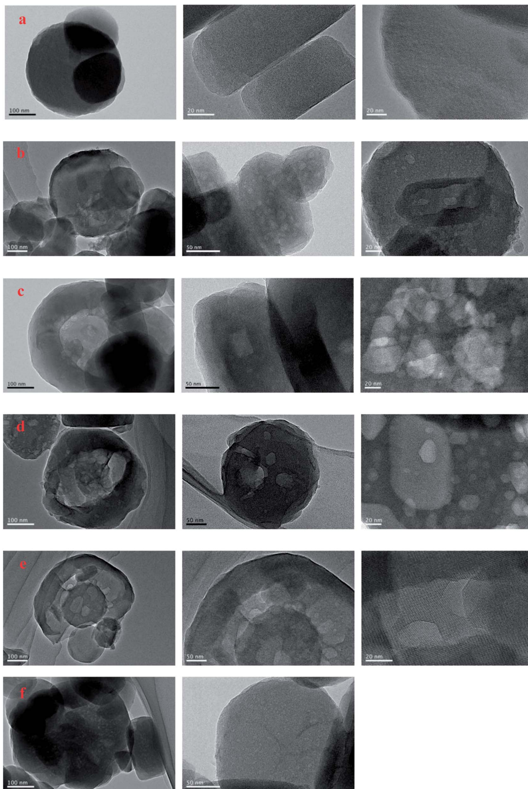
Fig. 3 TEM images of the parent, TEAOH-treated H-ZSM-5 and TPA-16 h samples ((a) parent H-ZSM-5, (b) T-4 h, (c) T-16 h, (d) T-24 h, (e) T-48 h, (f) TEA-16 h).
