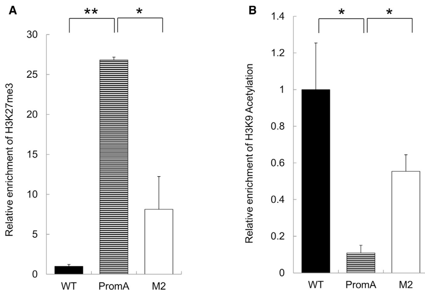
Figure 5. shPromA Suppressed Viral Replication through TGS
