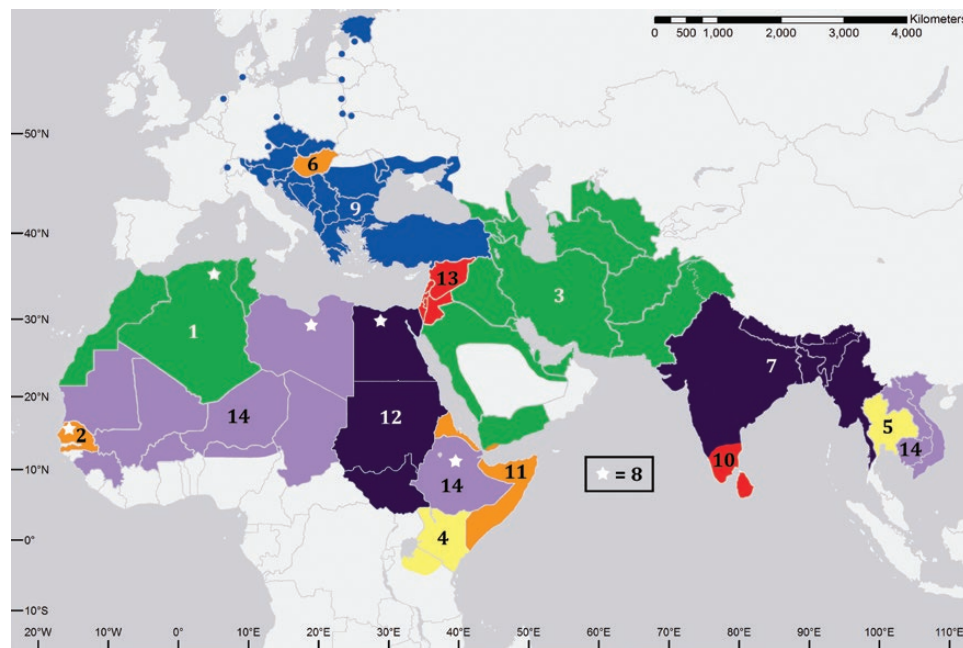
Fig. 3. —Geographic distribution of Canis aureus includes subspecies that may belong to C. anthus or C. lupus . The map shows the likely ranges of the following subspecies, 1, C. a. algirensis ; 2, C. a. anthus ; 3, C. a. aureus ; 4, C. a. bea ; 5, C. a. cruesmanni ; 6, C. a. ecsedensis ; 7, C. a. indicus ; 8, C. a. lupaster (dispersed stars on map); 9, C. a. moreotica (isolated records presented as blue dots on map); 10, C. a. naria ; 11, C. a. riparius ; 12, C. a. soudanicus ; 13, C. a. syriacus ; 14, C. a. subspecies undetermined.
