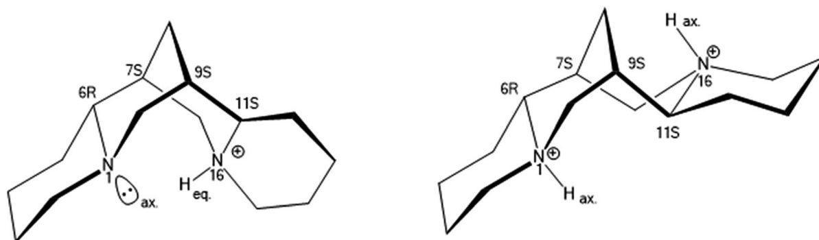
Fig. 6 Spatial relationship of mono and diprotonated sparteinium cations, [\text{HSpa}]^+ and [\text{H}_2\text{Spa}]^{2+} showing shape change.
